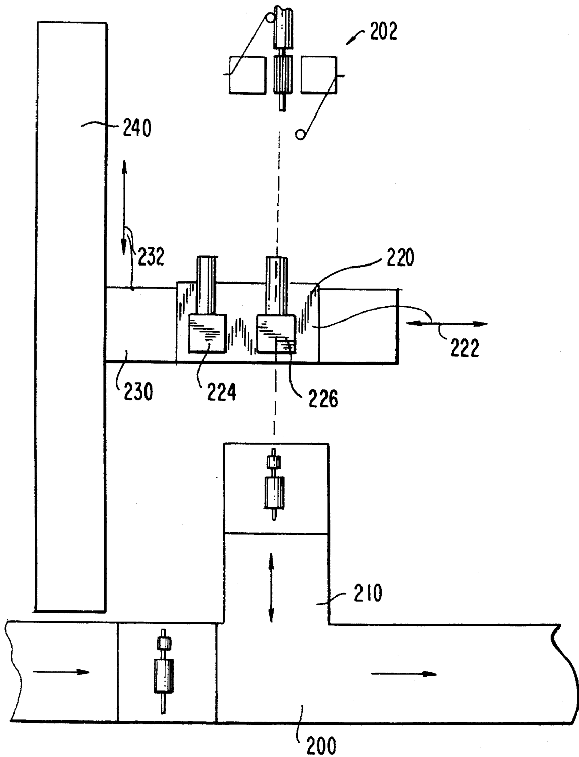
FIG. 2 PRIOR ART
