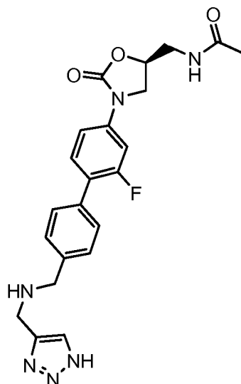
radezolid
