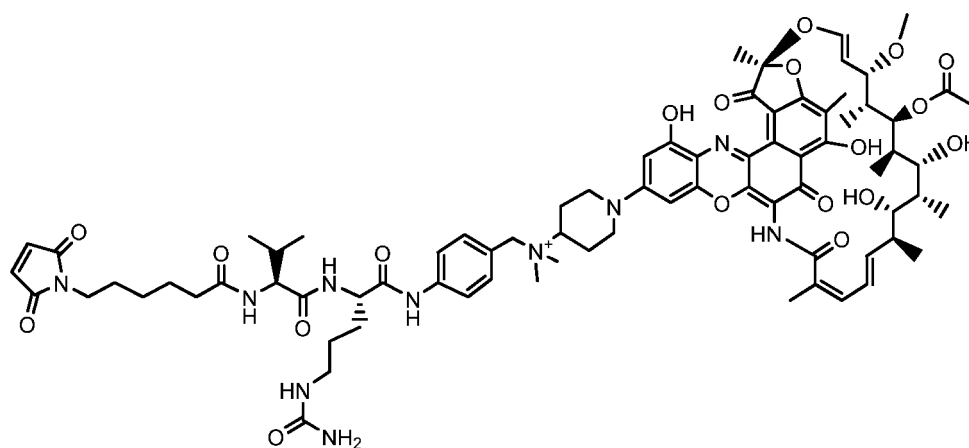
MC-vc-PAB-(dimethylpipBOR)
