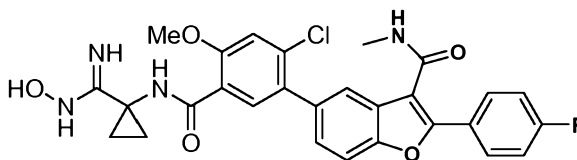
5-(2-Chloro-5-(1-(N-hydroxycarbamimidoyl)cyclopropylcarbamoyl)-4-methoxyphenyl)-2-(4-fluorophenyl)-N-methylbenzofuran-3-carboxamide
