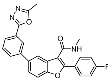
2-(4-Fluorophenyl)-N-methyl-5-(3-(5-methyl-1,3,4-oxadiazol-2-yl)phenyl)benzofuran-3-carboxamide
