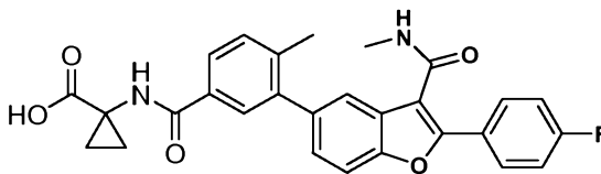
1-(3-(2-(4-Fluorophenyl)-3-(methylcarbamoyl)benzofuran-5-yl)-4-methylbenzamido)cyclopropanecarboxylic acid
