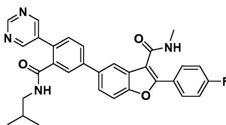
2-(4-Fluorophenyl)-5-(3-(isobutylcarbamoyl)-4-(pyrimidin-5-yl)phenyl)-N-methylbenzofuran-3-carboxamide
