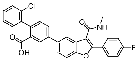
2'-Chloro-4-(2-(4-fluorophenyl)-3-(methylcarbamoyl)benzofuran-5-yl)biphenyl-2-carboxylic acid
