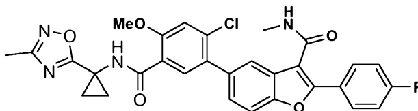
5-(2-Chloro-4-methoxy-5-(1-(3-methyl-1,2,4-oxadiazol-5-yl)cyclopropylcarbamoyl)phenyl)-2-(4-fluorophenyl)-N-methylbenzofuran-3-carboxamide
