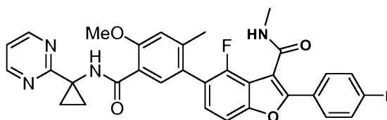
4-Fluoro-2-(4-fluorophenyl)-5-(4-methoxy-2-methyl-5-(1-(pyrimidin-2-yl)cyclopropylcarbamoyl)phenyl)-N-methylbenzofuran-3-carboxamide
