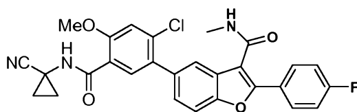
5-(2-Chloro-5-(1-cyanocyclopropylcarbamoyl)-4-methoxyphenyl)-2-(4-fluorophenyl)-N-methylbenzofuran-3-carboxamide
