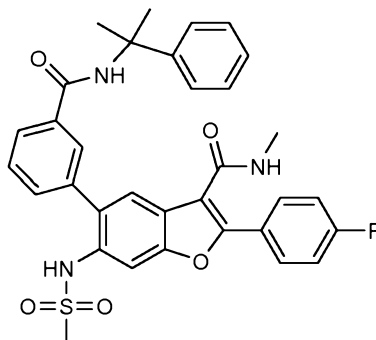
2-(4-Fluorophenyl)-N-methyl-6-(methylsulfonylamino)-5-(3-(2-phenylpropan-2-ylcarbamoyl)phenyl)benzofuran-3-carboxamide
