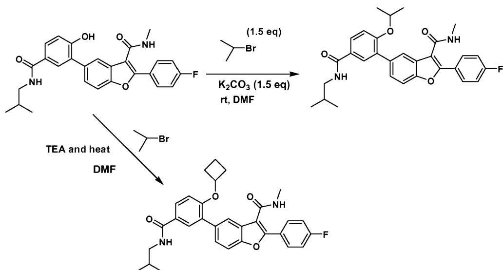
Scheme 9
