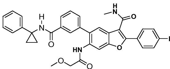
2-(4-Fluorophenyl)-6-(2-methoxyacetamido)-N-methyl-5-(3-(1-phenylcyclopropylcarbamoyl)phenyl)benzofuran-3-carboxamide
