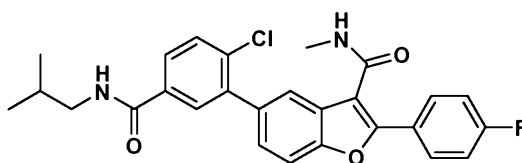
5-(2-Chloro-5-(isobutylcarbamoyl)phenyl)-2-(4-fluorophenyl)-N-methylbenzofuran-3-carboxamide
