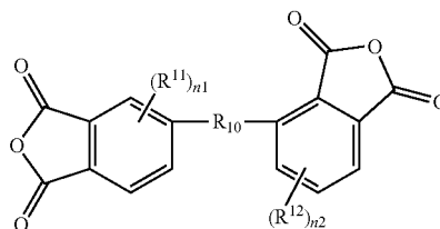
Chemical Formula 1-3
