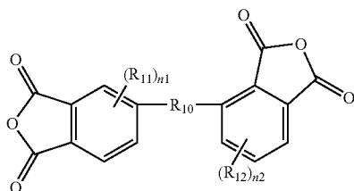
Chemical Formula 1-3
