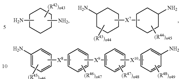
Chemical Formula 3
