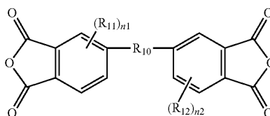
Chemical Formula 1-3
