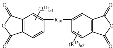
Chemical Formula 1-2
