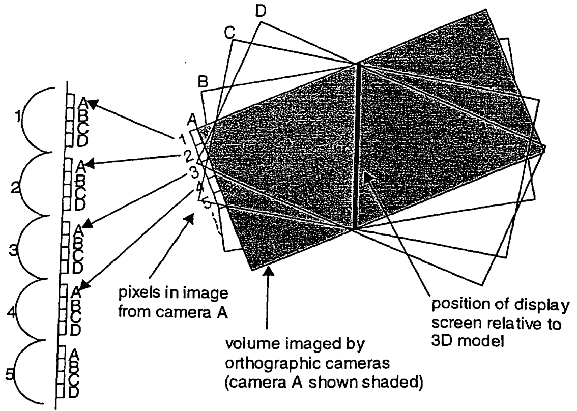
Microlenses and image obtained by multiplexing orthographic camera images
