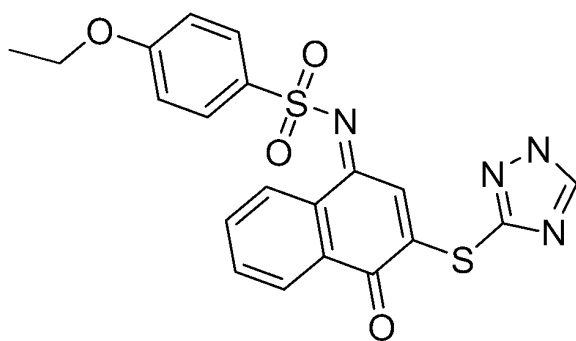
(Z)-N-(3-(1H-1,2,4-triazol-3-ylthio)-4-oxonaphthalen-1(4H)-ylidene)-4-ethoxybenzenesulfonamide
