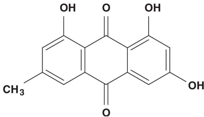
Emodin
