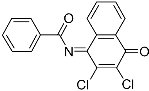
(E)-N-(2,3-dichloro-4-oxonaphthalen-1(4H)-ylidene)benzamide
