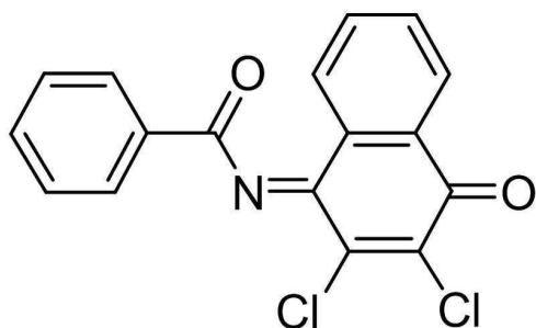
(E)-N-(2,3-dichloro-4-oxonaphthalen-1(4H)-ylidene)benzamide
