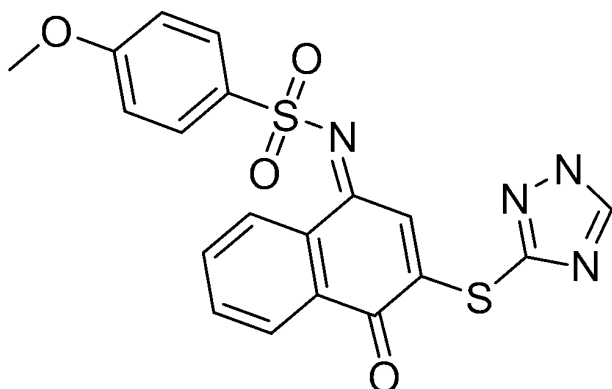
(Z)-N-(3-(1H-1,2,4-triazol-3-ylthio)-4-oxonaphthalen-1(4H)-ylidene)-4-methoxybenzenesulfonamide
