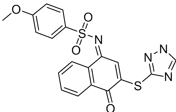
(Z)-N-(3-(1H-1,2,4-triazol-3-ylthio)-4-oxonaphthalen-1(4H)-ylidene)-4-methoxybenzenesulfonamide
