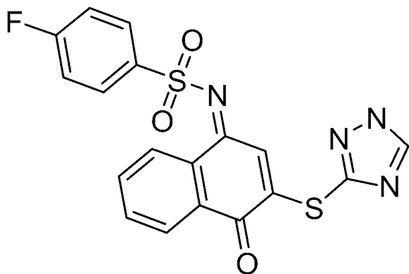
(Z)-N-(3-(1H-1,2,4-triazol-3-ylthio)-4-oxonaphthalen-1(4H)-ylidene)-4-fluorobenzenesulfonamide
