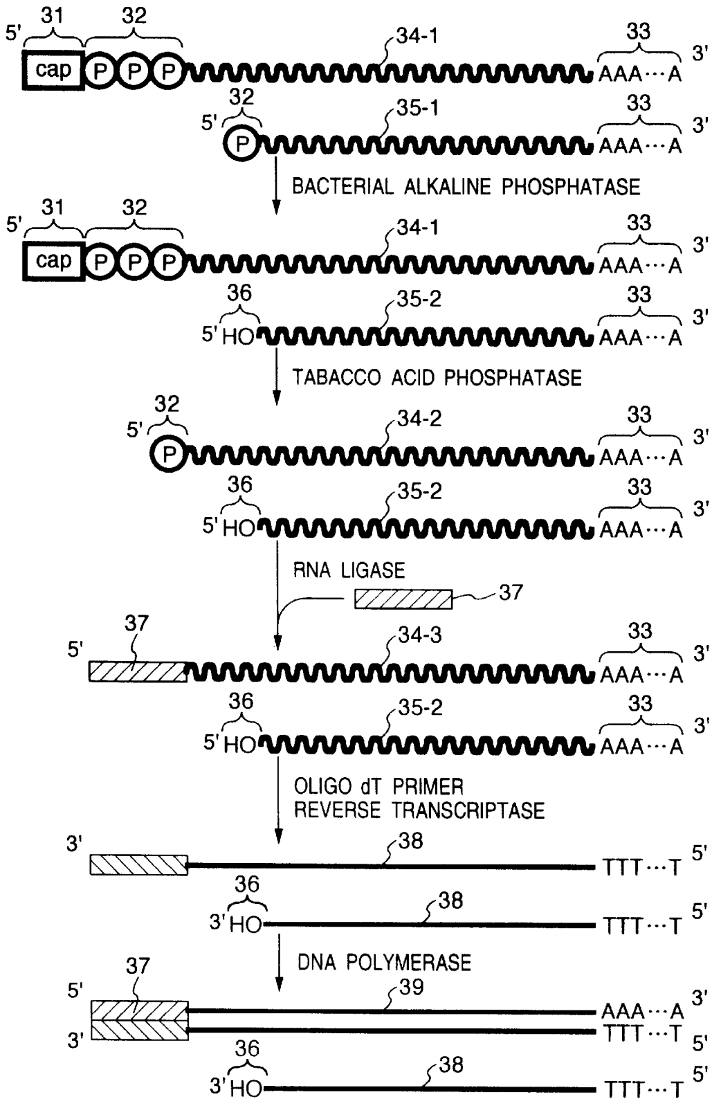
FIG. 3 PRIOR ART
