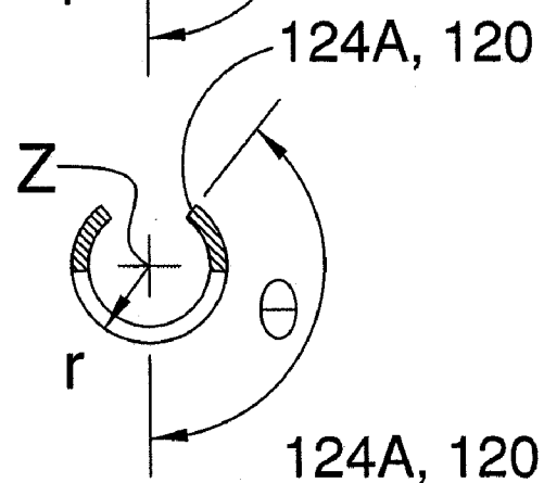
FIG. 6C SECTION F-F
