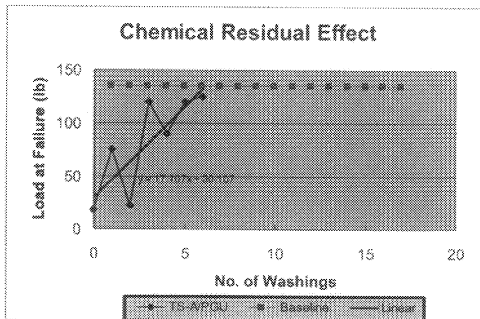
Figure 10. Bond Strength Reduction -- TS-A/PGU. Quarry Tile - Absorptivity = 0.27
