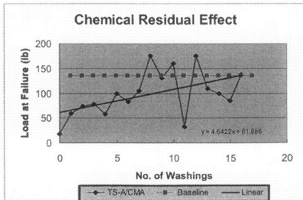
Figure 8. Bond Strength Reduction -- TS-A/CMA. Quarry Tile - Absorptivity = 0.27
