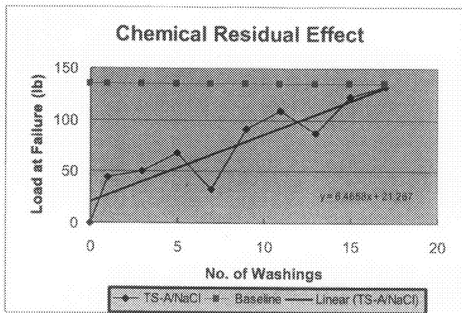
Figure 11. Bond Strength Reduction -- TS-A/NaCl. Quarry Tile - Absorptivity = 0.27
