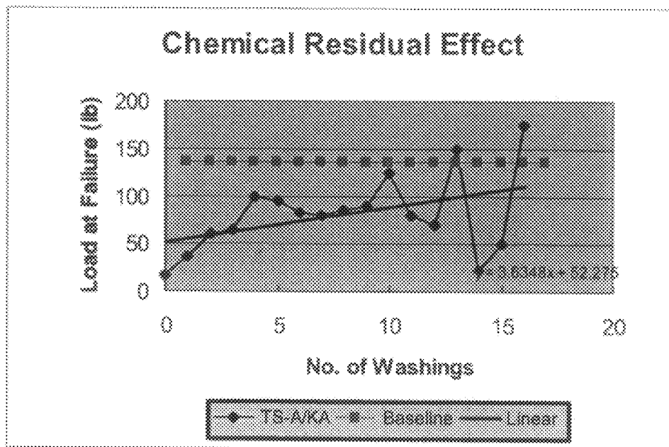
Figure 9. Bond Strength Reduction -- TS-A/KA. Quarry Tile - Absorptivity = 0.27
