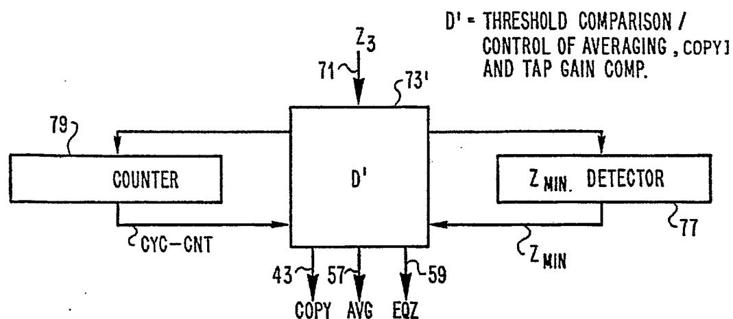
FIG. 5 ALTERNATIVE EVALUATION AND CONTROL MEANS
