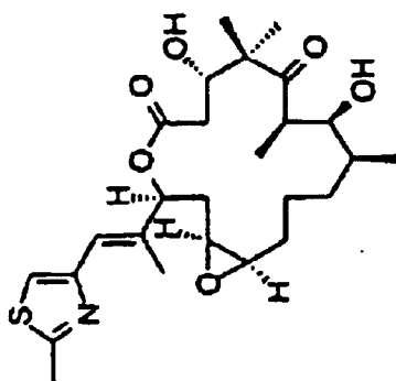
epothilone A
