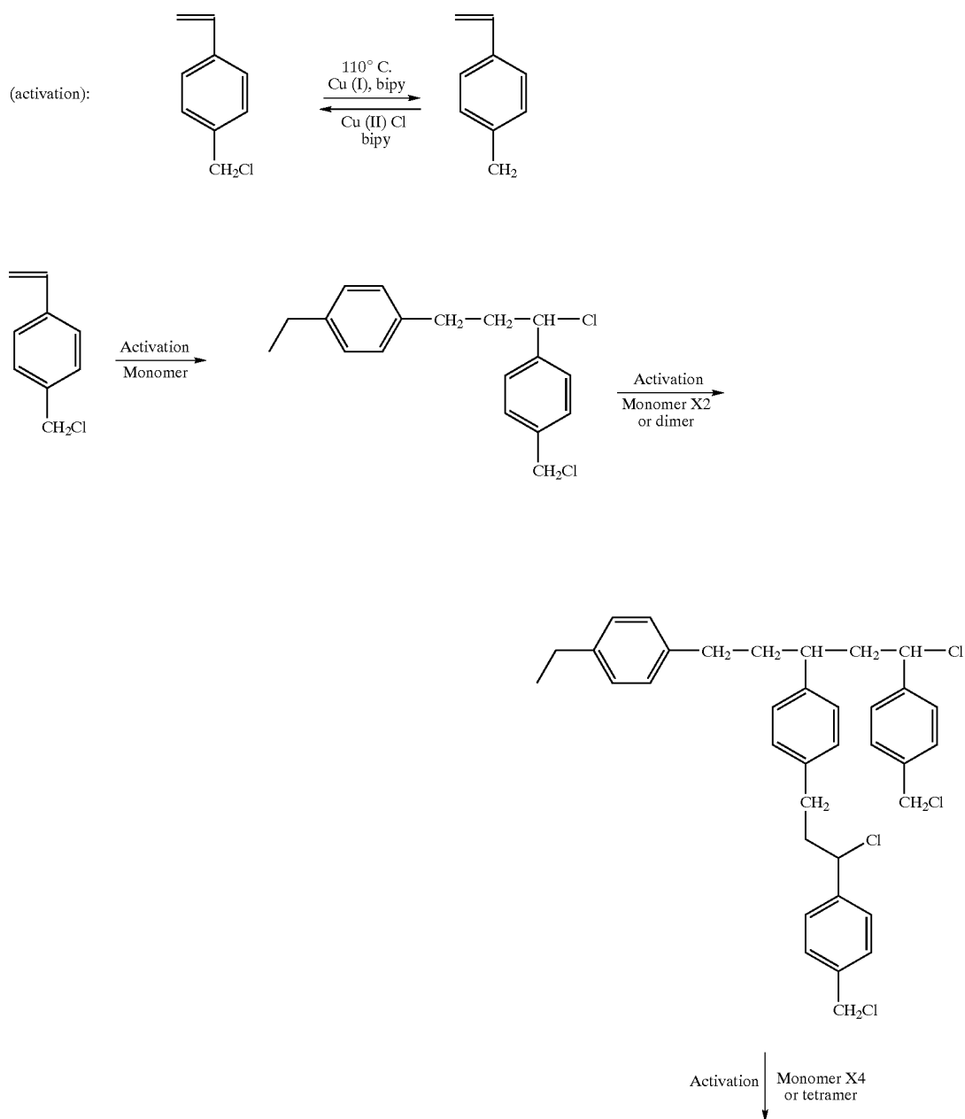
Scheme 3
