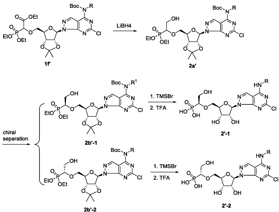
Scheme 3
