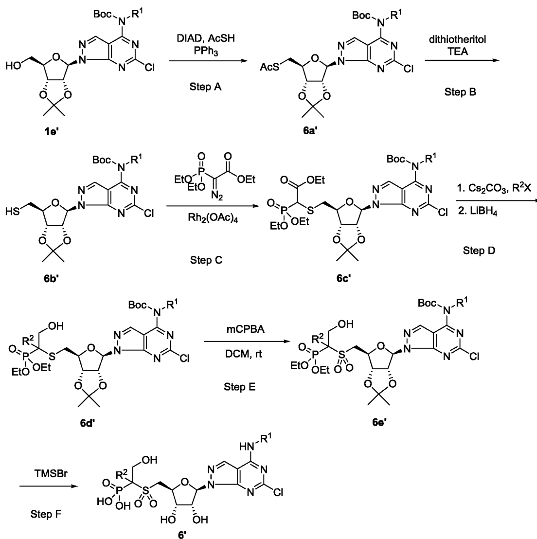
Scheme 7
