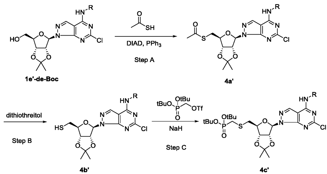
Scheme 5
