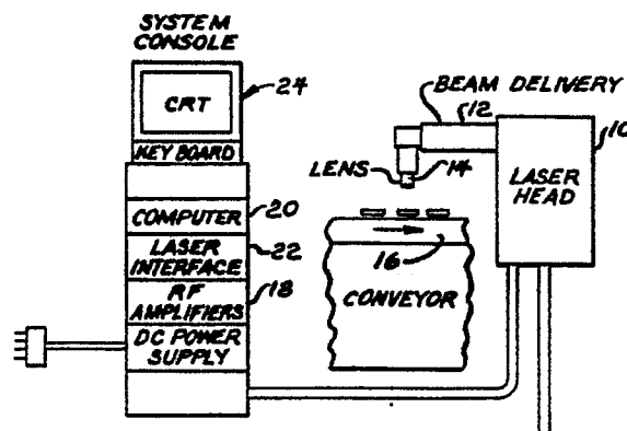
SYSTEM CONFIGURATION FIG. 1
