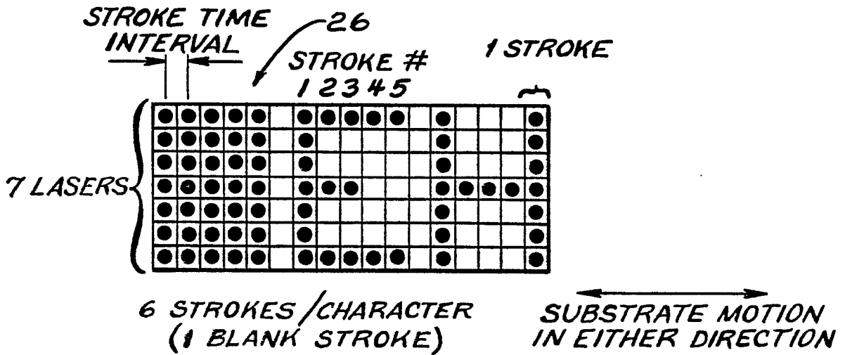
5x7 DOT MATRIX FIG. 2
