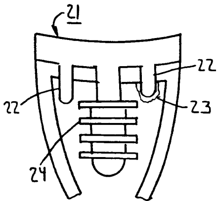
FIGURE 8 PRIOR ART
