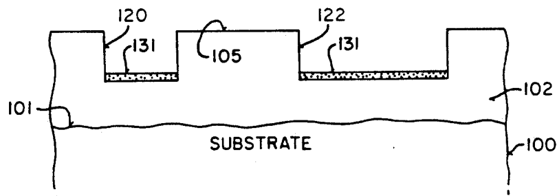
FIG 4 (PRIOR ART)
