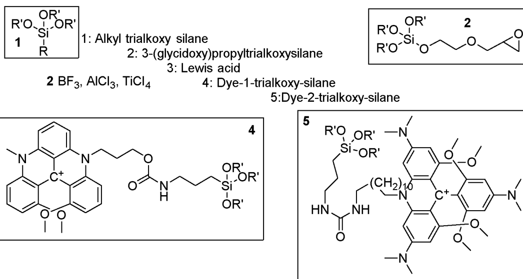
Scheme 1: Above is shown the five components used to form the sol-gel sensor material in the present example.
