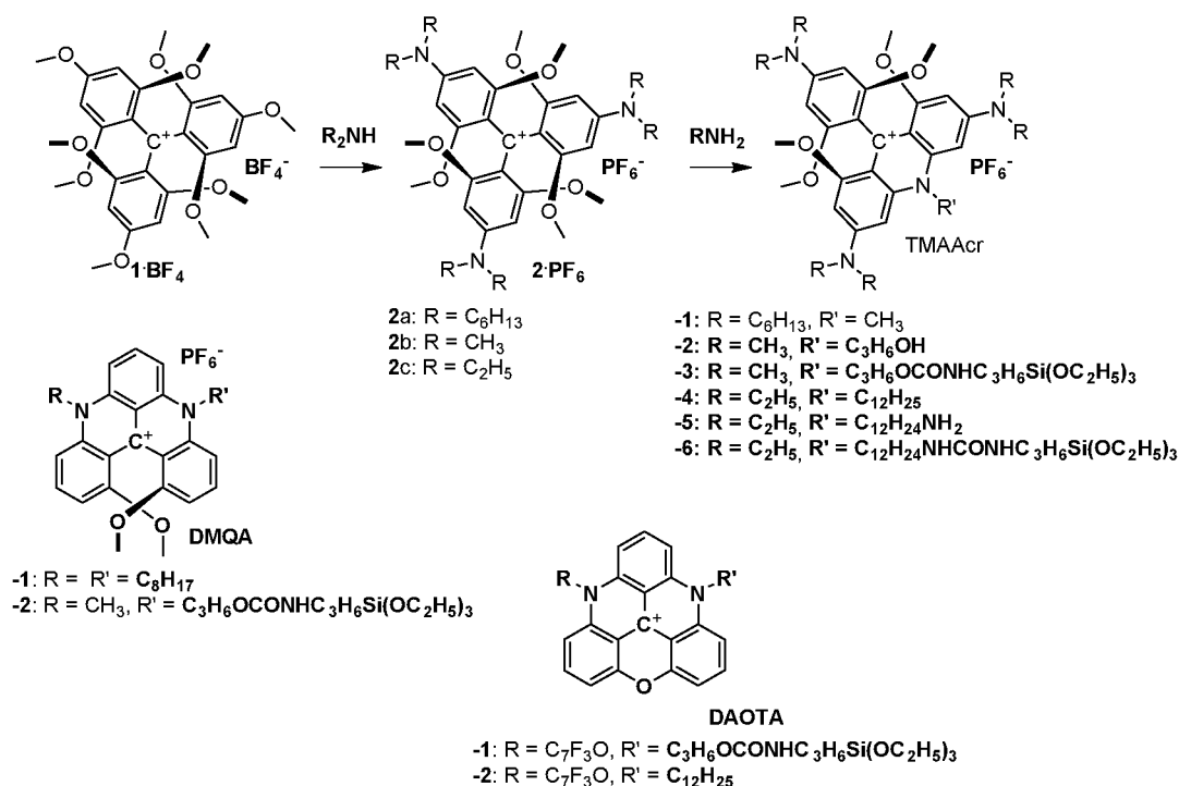
Scheme 2. Molecular structure of the pH responsive and the reference dyes.
