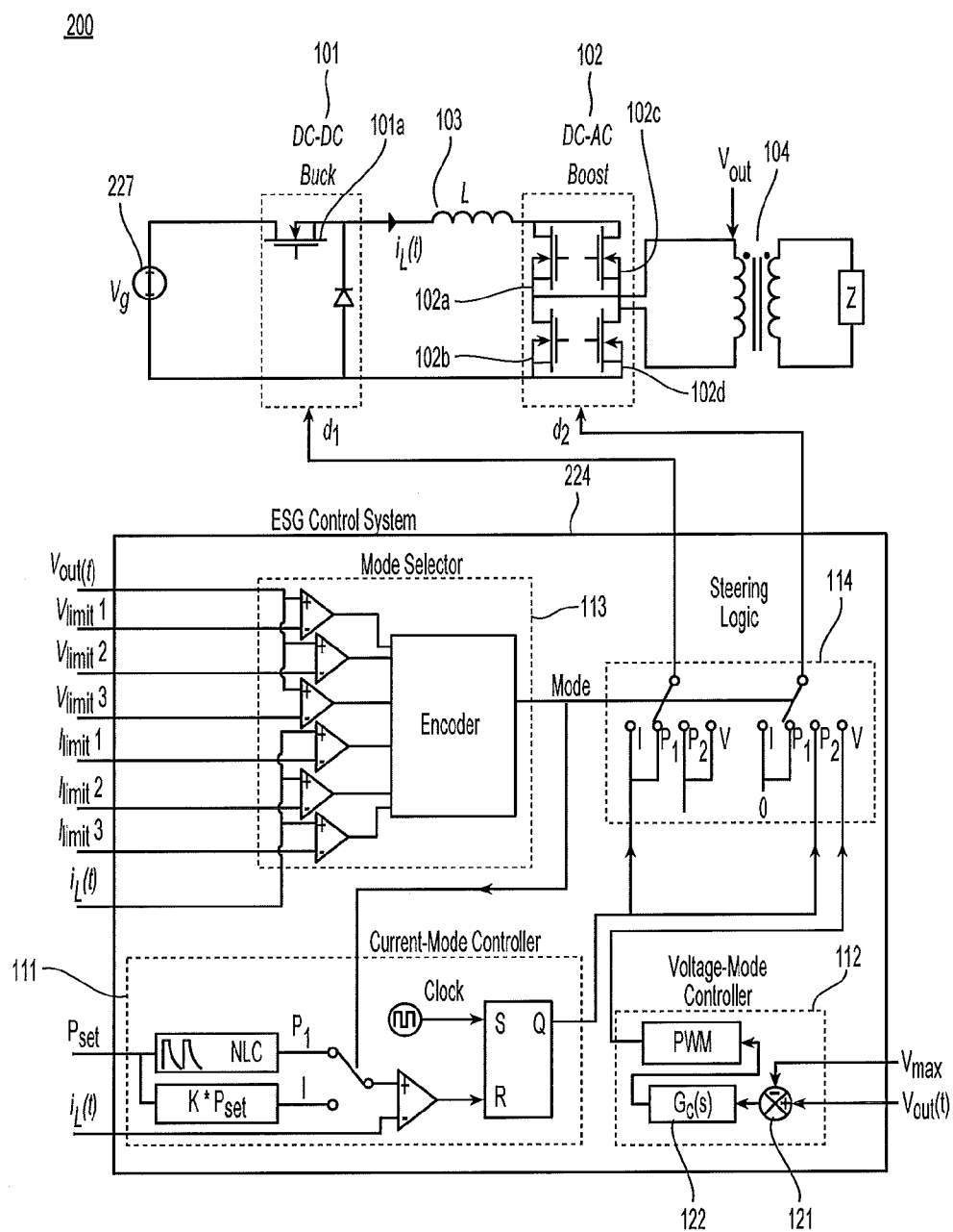
ESG including buck-derived constant power source
