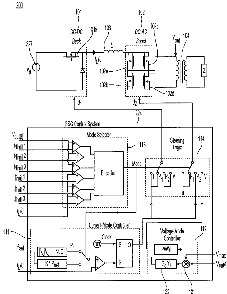
ESG including buck-derived constant power source
