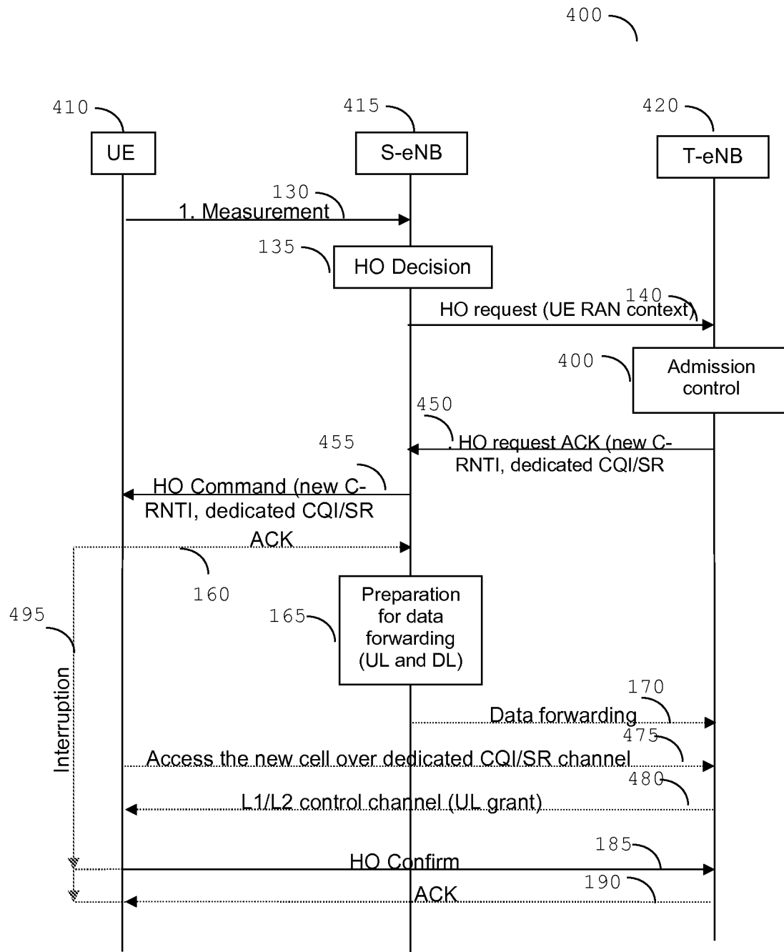
FIG. 4 PRIOR ART
