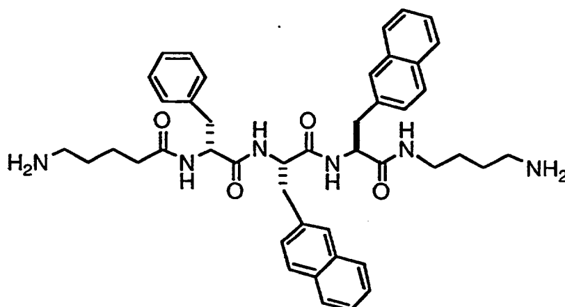
(5-Aminovaleryl)-DPhe-βNal-βNal-[N-(4-aminobutyl)] amide, TFA salt
