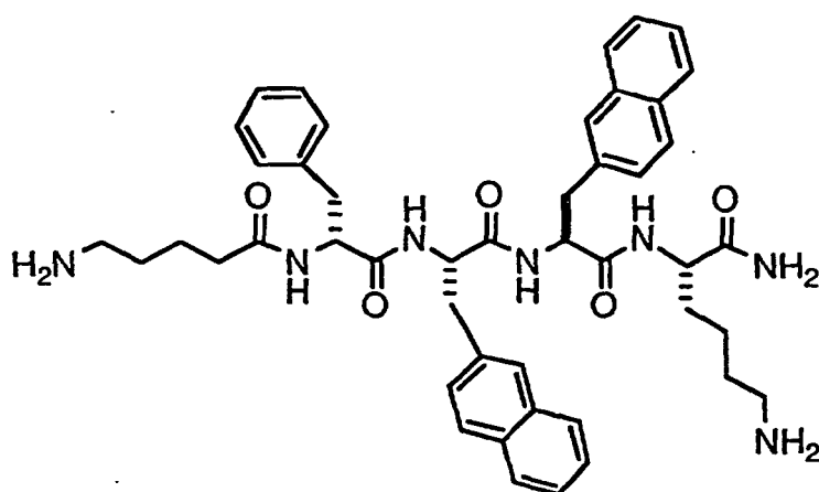
(5-Aminovaleryl)-DPhe-βNal-βNal-Lys-amide, TFA salt
