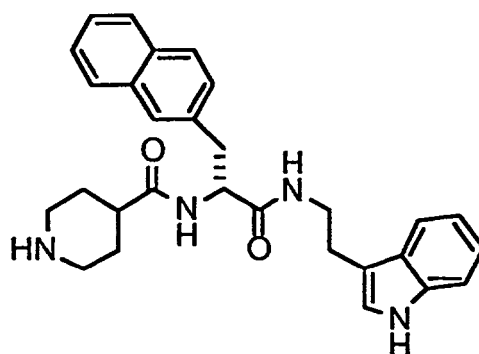
(inip)-DβNal-[N-tryptaminy] amide, TFA salt
