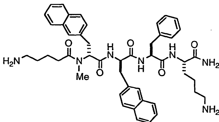
(5-Aminovaleryl)-(N-Me-D \beta Nal)-D \beta Nal-Phe-Lys-amide, TFA salt
