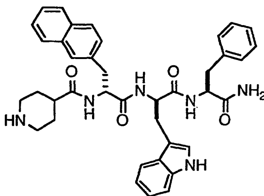
(inip)-D \beta Nal-DTrp-Phe-amide, TFA salt
