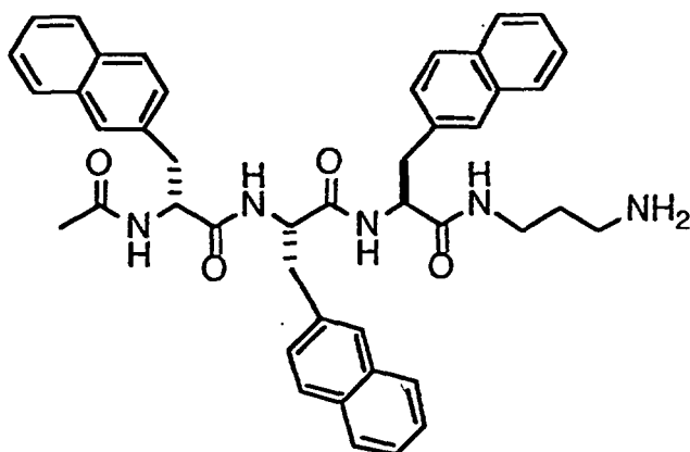
Acetyl-DβNal-βNal-βNal-[N-(3-aminopropyl)] amide, TFA salt
