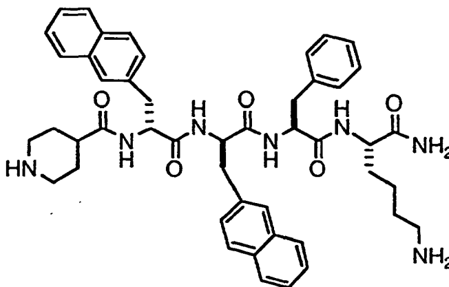
(inip)-D \beta Nal-D \beta Nal-Phe-Lys-amide, TFA salt
