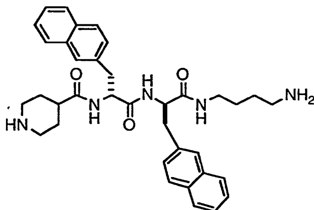
(inip)-DβNal-DβNal-[N-(4-aminobutyl)] amide, TFA salt
