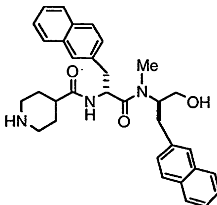
(inip)-DβNal-(N-Methyl-D-β-naphthylalanol), TFA salt
