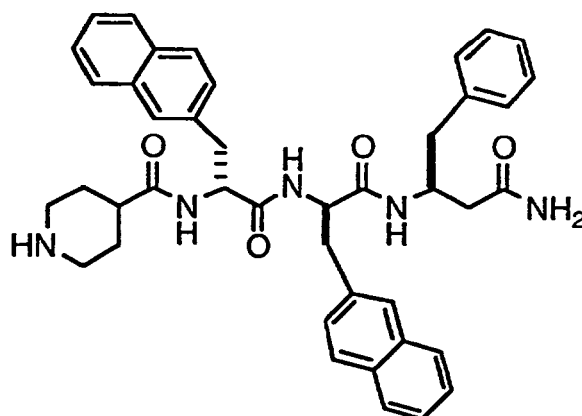
(inip)-D \beta Nal-D \beta Nal-(3(S)-3-benzyl- \beta -Ala) amide, TFA salt
