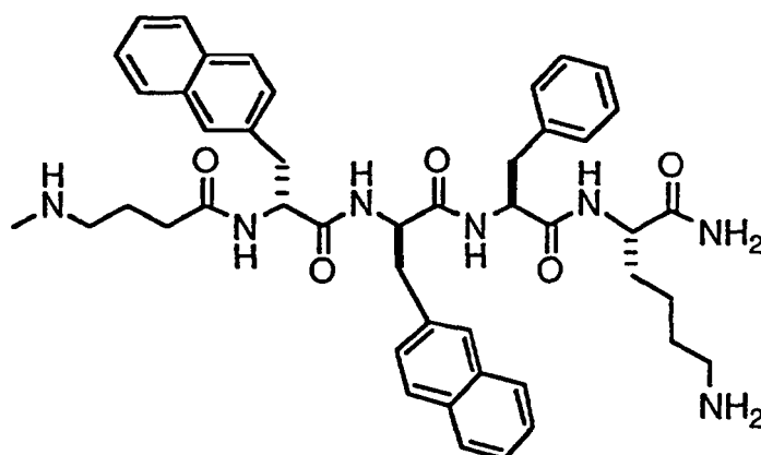
[4-(N-Methylamino)butanoyl]-DβNal-DβNal-Phe-Lys-amide, TFA salt
