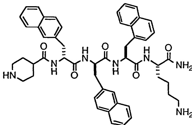
(inip)-DβNal-DβNal-αNal-Lys-amide, TFA salt
