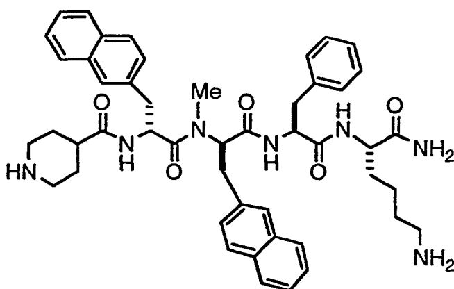
(inip)-D \beta Nal-(N-Me-D \beta Nal)-Phe-Lys-amide, TFA salt
