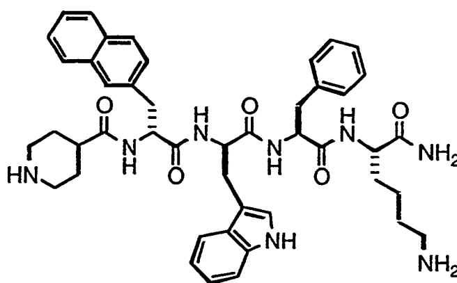
(inip)-DβNal-DTrp-Phe-Lys-amide, TFA salt
