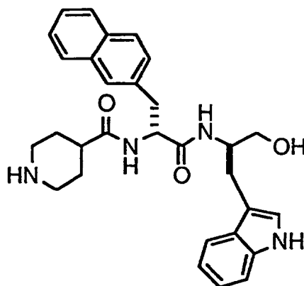
(inip)-DβNal-(D-Tryptophanol), TFA salt
