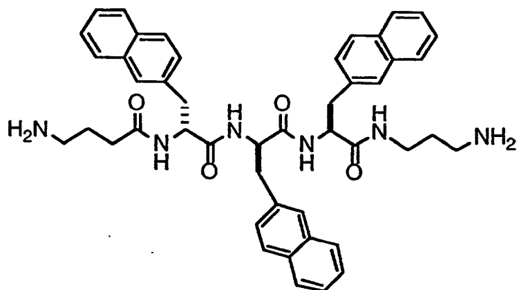
(4-Aminobutanoyl)-DβNal-DβNal-βNal-[N-(3-aminopropyl)] amide, TFA salt
