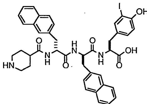
(inip)-D \beta Nal-D \beta Nal-(3-I-Tyr), TFA salt
