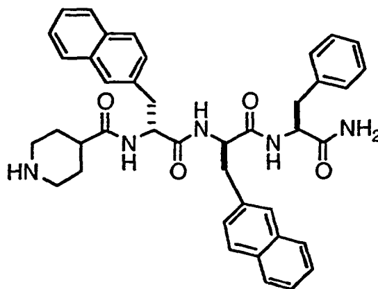
(inip)-D \beta Nal-D \beta Nal-Phe-amide, TFA salt
