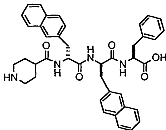
(inip)-DβNal-DβNal-Phe, TFA salt
