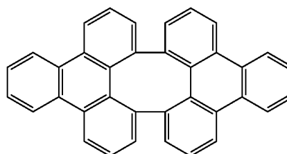
1, 12-fused-BT
