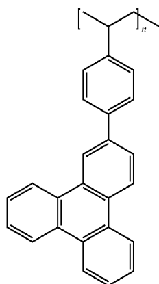
Synthesis of poly(2,7-triphenylene)
