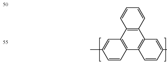
Synthesis of poly(2,7-triphenylene-1,4-phenylene)
