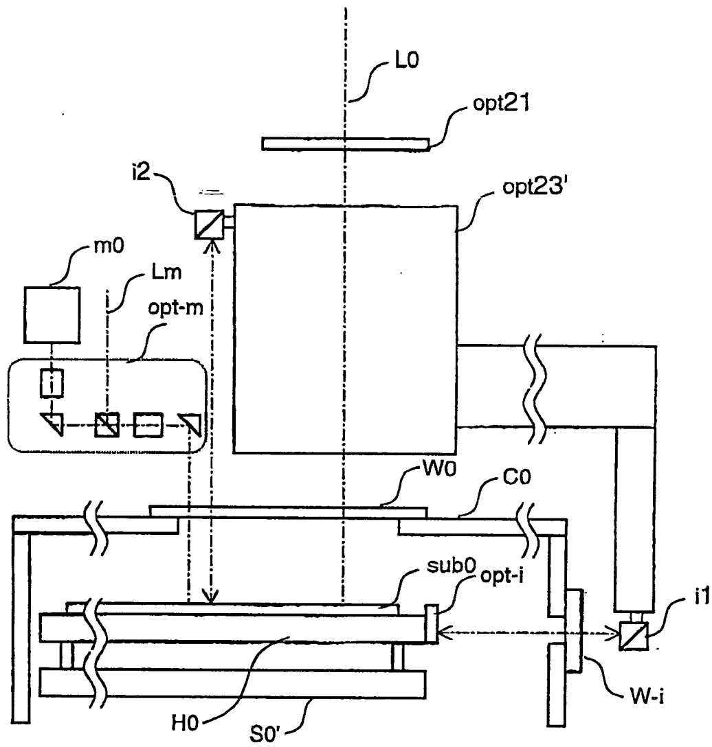
ALIGNMENT MECHANISM
