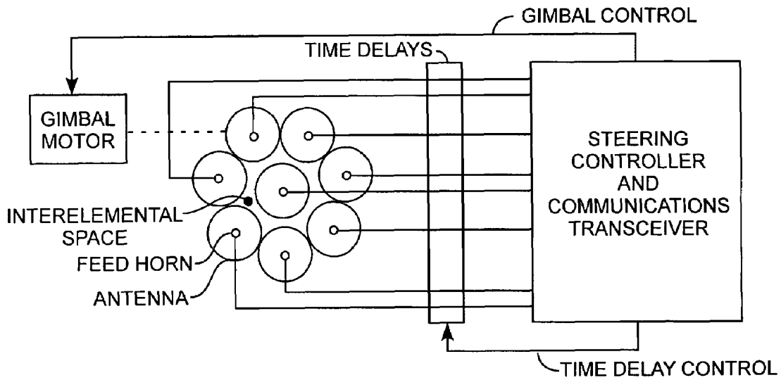
HEPTAGONAL ANTENNA ARRAY SYSTEM FIG. 1
