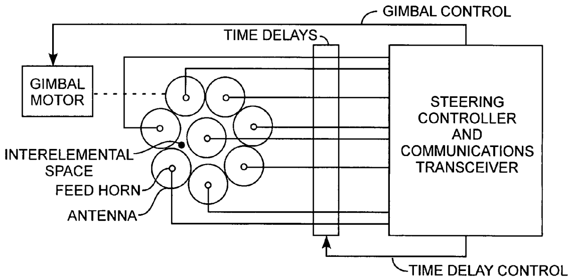
HEPTAGONAL ANTENNA ARRAY SYSTEM
