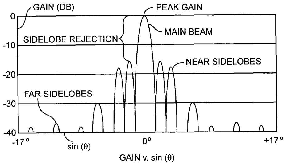
HEPTAGONAL ANTENNA PERFORMANCE FIG. 2
