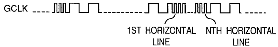
Fig.33C RELATED ART
