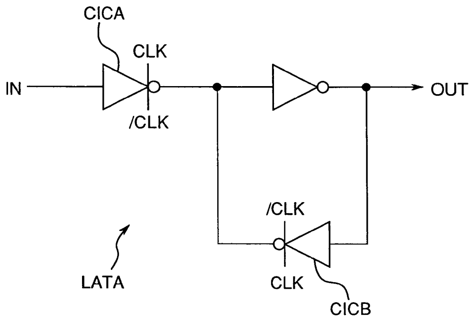
Fig.26 RELATED ART
