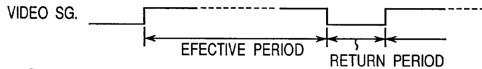
Fig.33C RELATED ART
