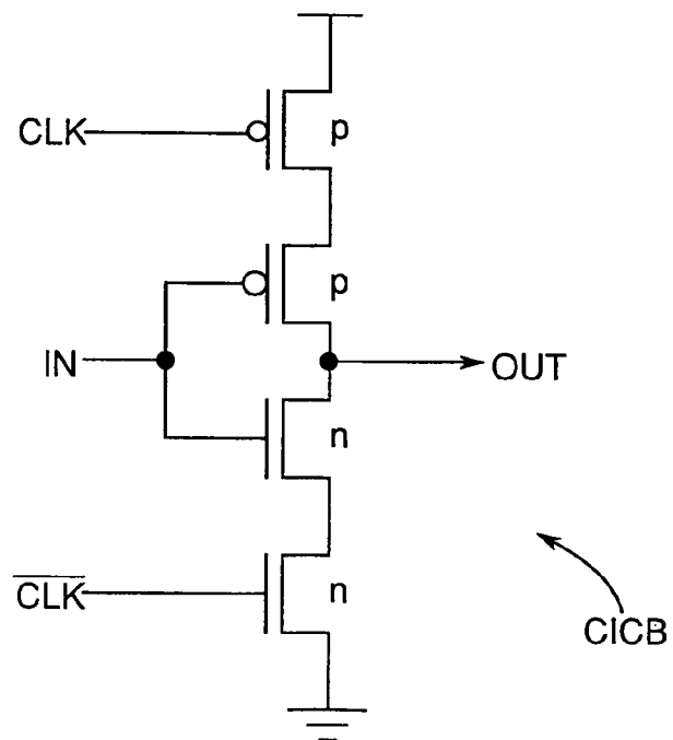
Fig.29 RELATED ART
