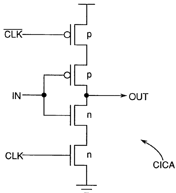
Fig.28 RELATED ART
