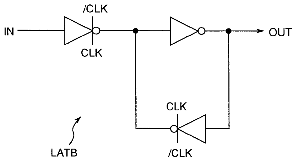
Fig.27 RELATED ART
