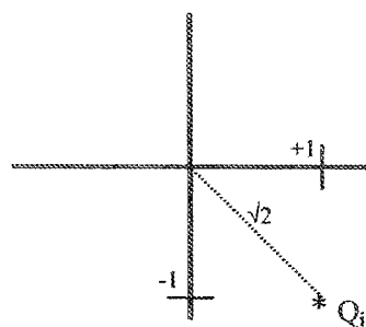
Q-Mode {+,-} Constellation Point Fig. 2
