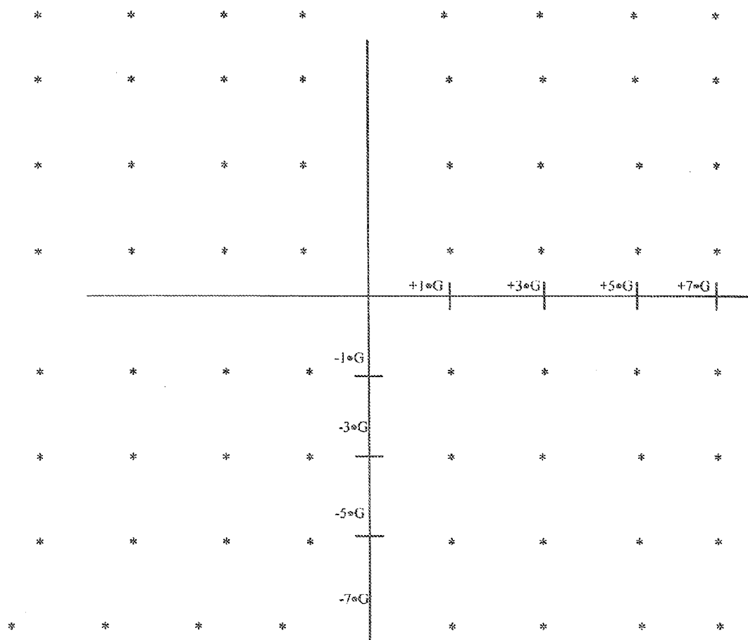
64-QAM Constellation Fig. 3
