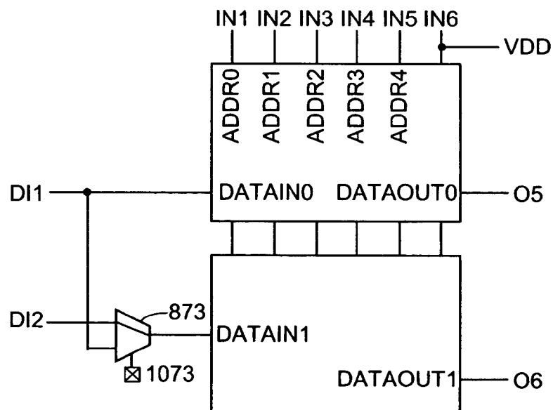
FIG. 11 (32x2 RAM)
