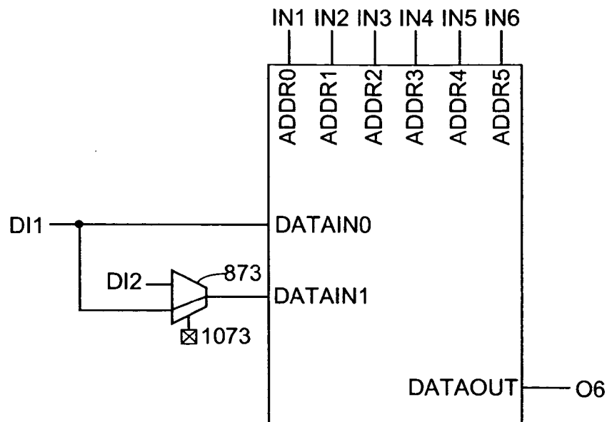
FIG. 10 (64x1 RAM)
