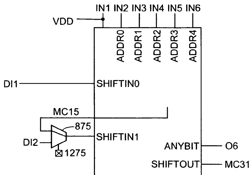
FIG. 12 (32x1 SRL)
