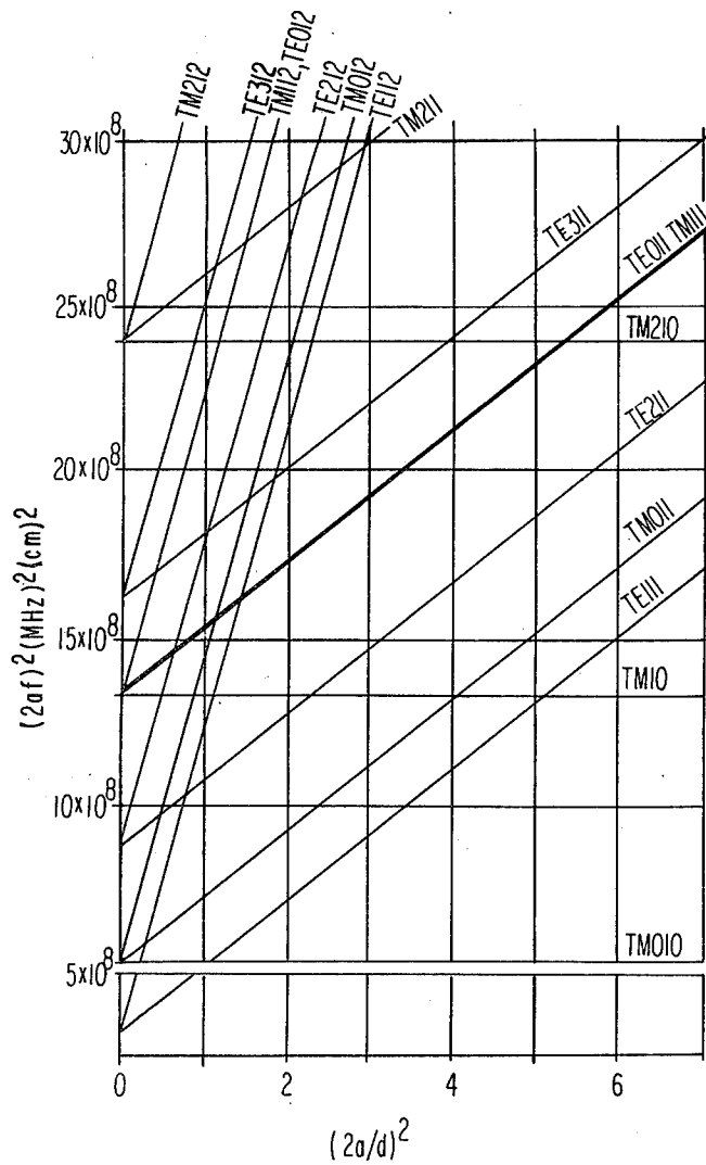
CIRCULAR CYLINDRICAL MODE CHART
