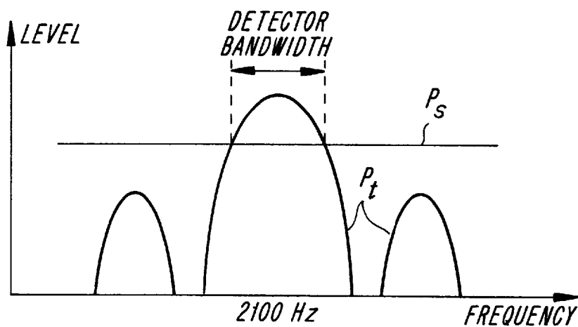
Fig. 2 (PRIOR ART)
