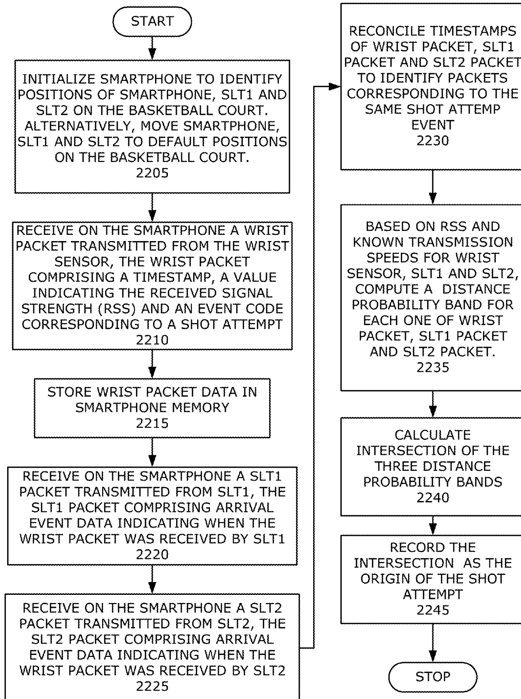
FIG. 22 - SHOT ATTEMPT LOCATION ALGORITHM
