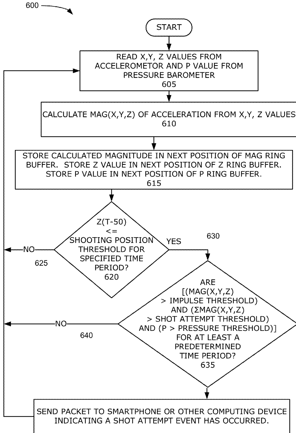
FIG. 6 - WRIST TRACKER SHOT-ATTEMPT ALGORITHM
