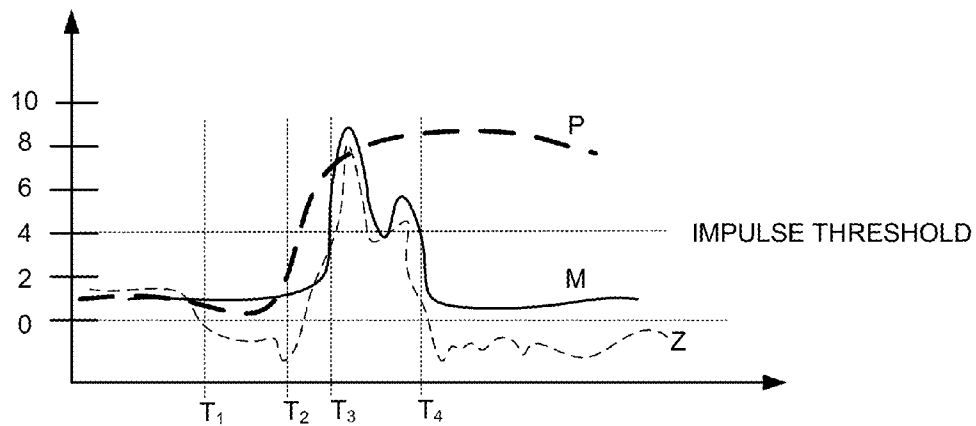
FIG. 5B - SHOT ATTEMPT PROFILE
