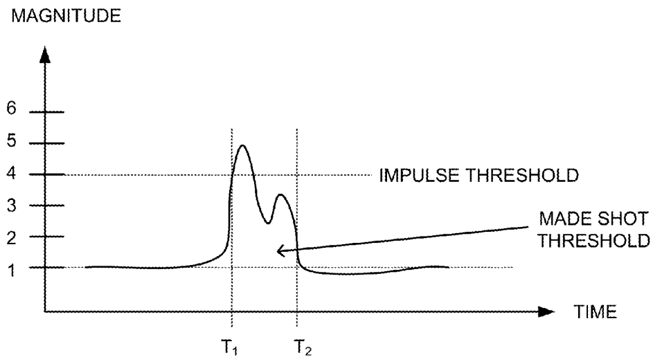
FIG. 11A MADE SHOT ACCELERATION PROFILE
