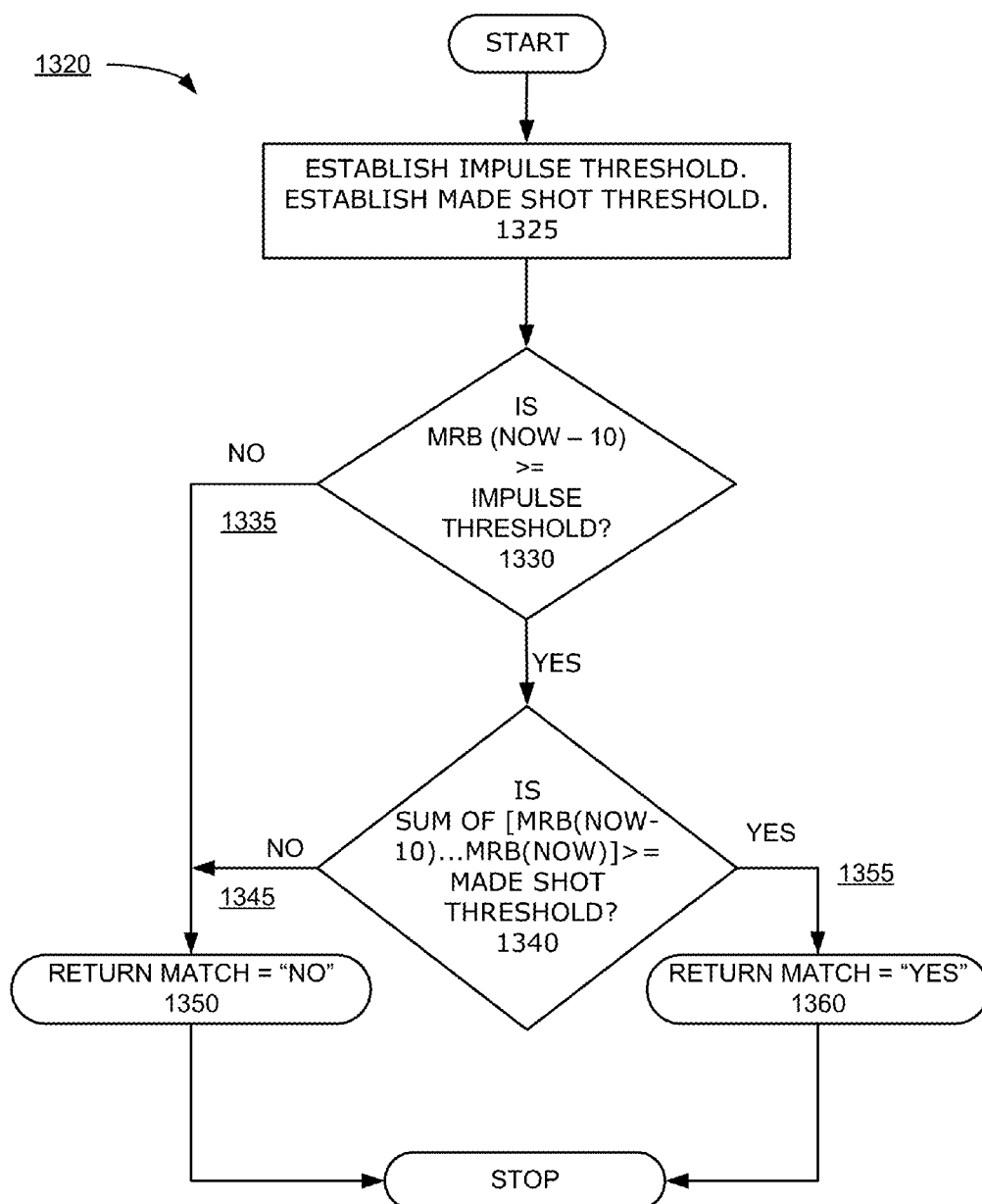
FIG. 13 PATTERN MATCHING ALGORITHM FOR NET TRACKER
