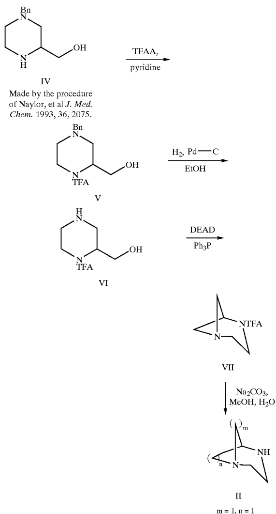
Scheme II
