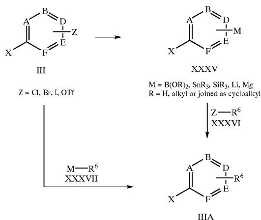
Scheme IX
