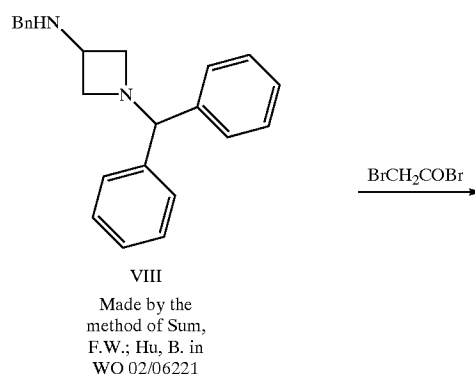
Scheme III
