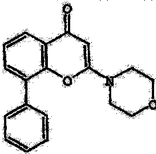
LY294002
