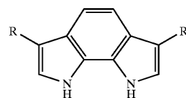
11a: R = H 11b: R = methyl 11c: R = dimethylamino-methyl
