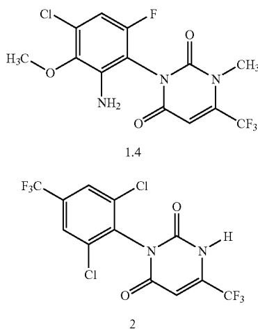
Comparative herbicidal activity of compounds 1.4 and 2
