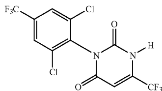
Comparative herbicidal activity of compounds 1.4 and 2
