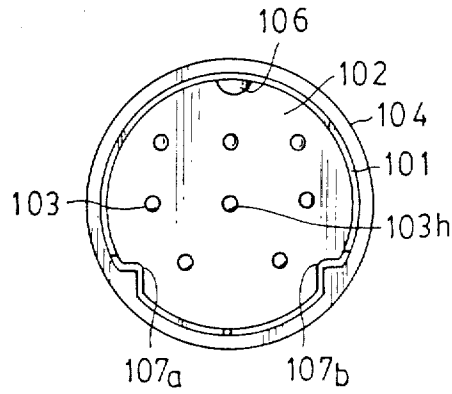
FIG. 4 PRIOR ART
