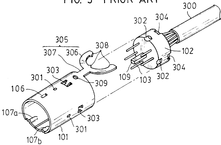
FIG. 5 PRIOR ART
