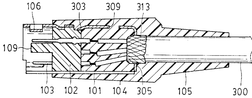
FIG. 6 PRIOR ART
