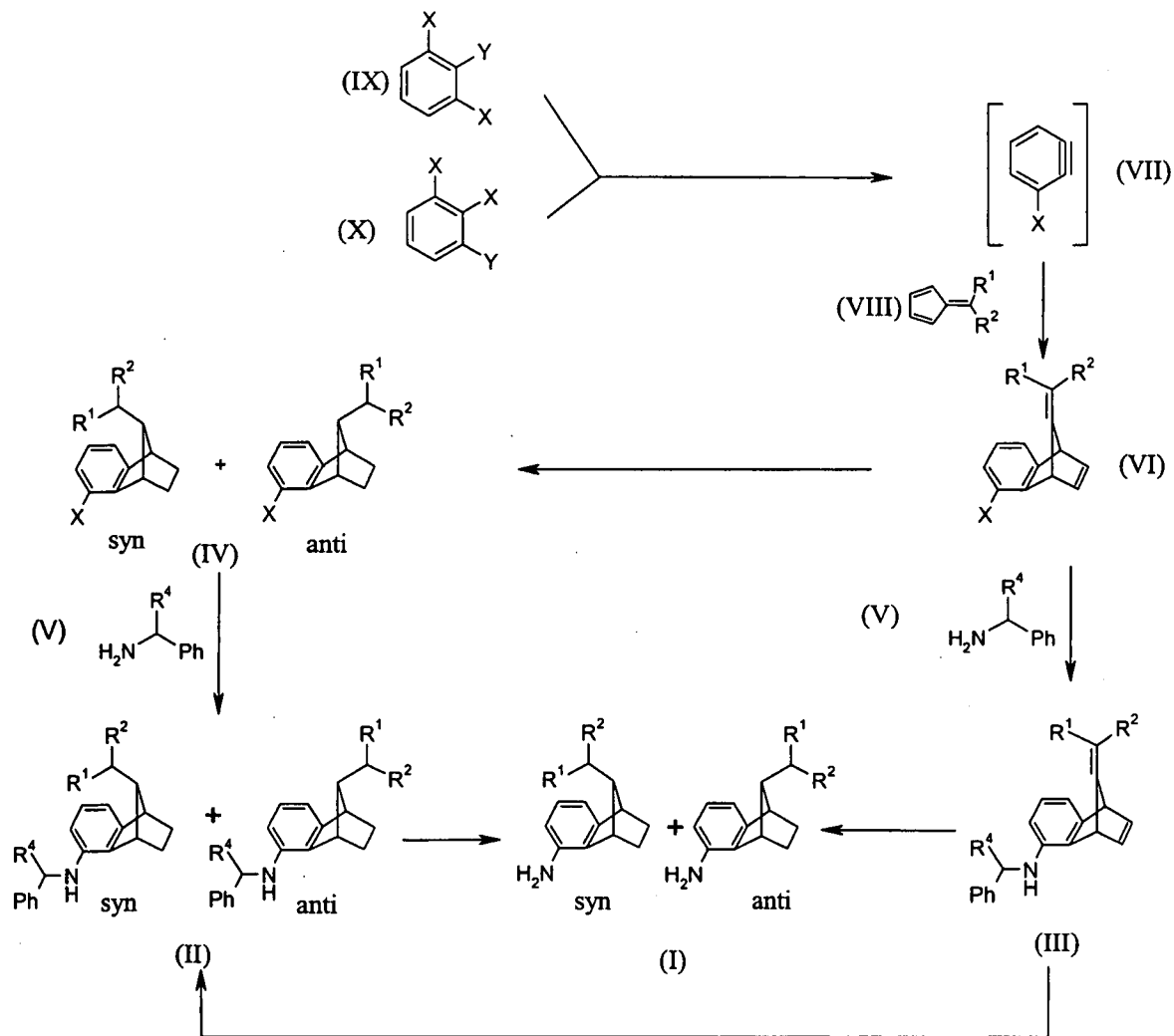
Scheme 2
