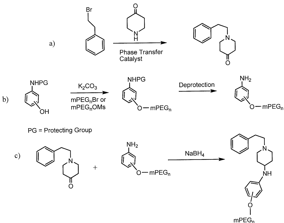
Scheme 4-C
