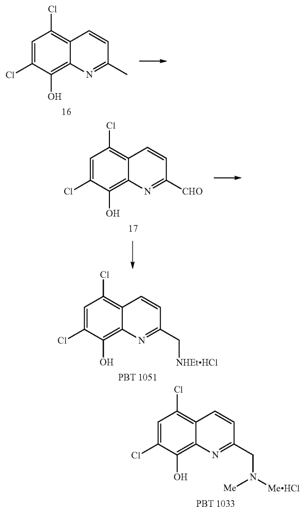
Scheme 15
