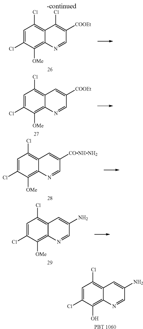
4,5,7-Trichloro-8-methoxy-quinoline-3-carboxylic acid ethyl ester 26
