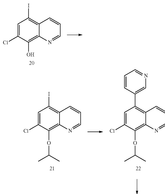
Scheme 17
