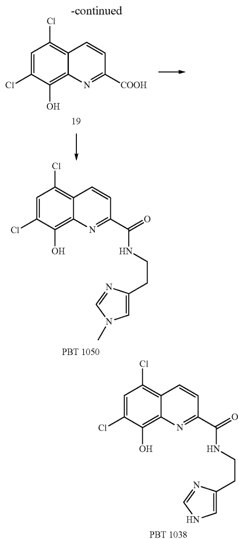
5,7-Dichloro-8-hydroxyquinoline-2-carboxylic acid 19
