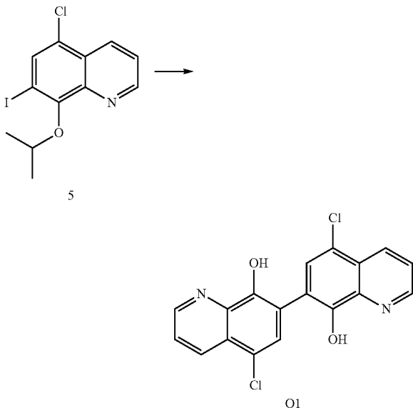
Scheme 11
