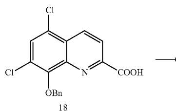
Scheme 16
