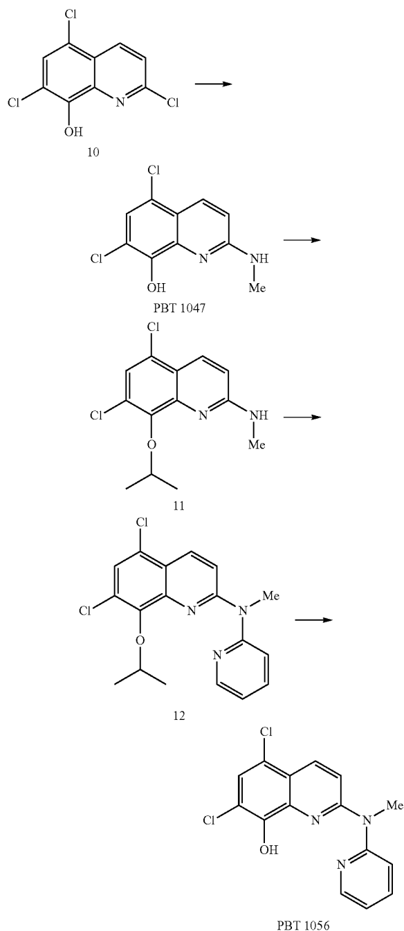
Scheme 13
