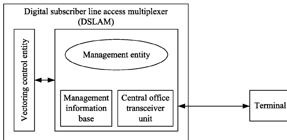
FIG. 1c PRIOR ART
