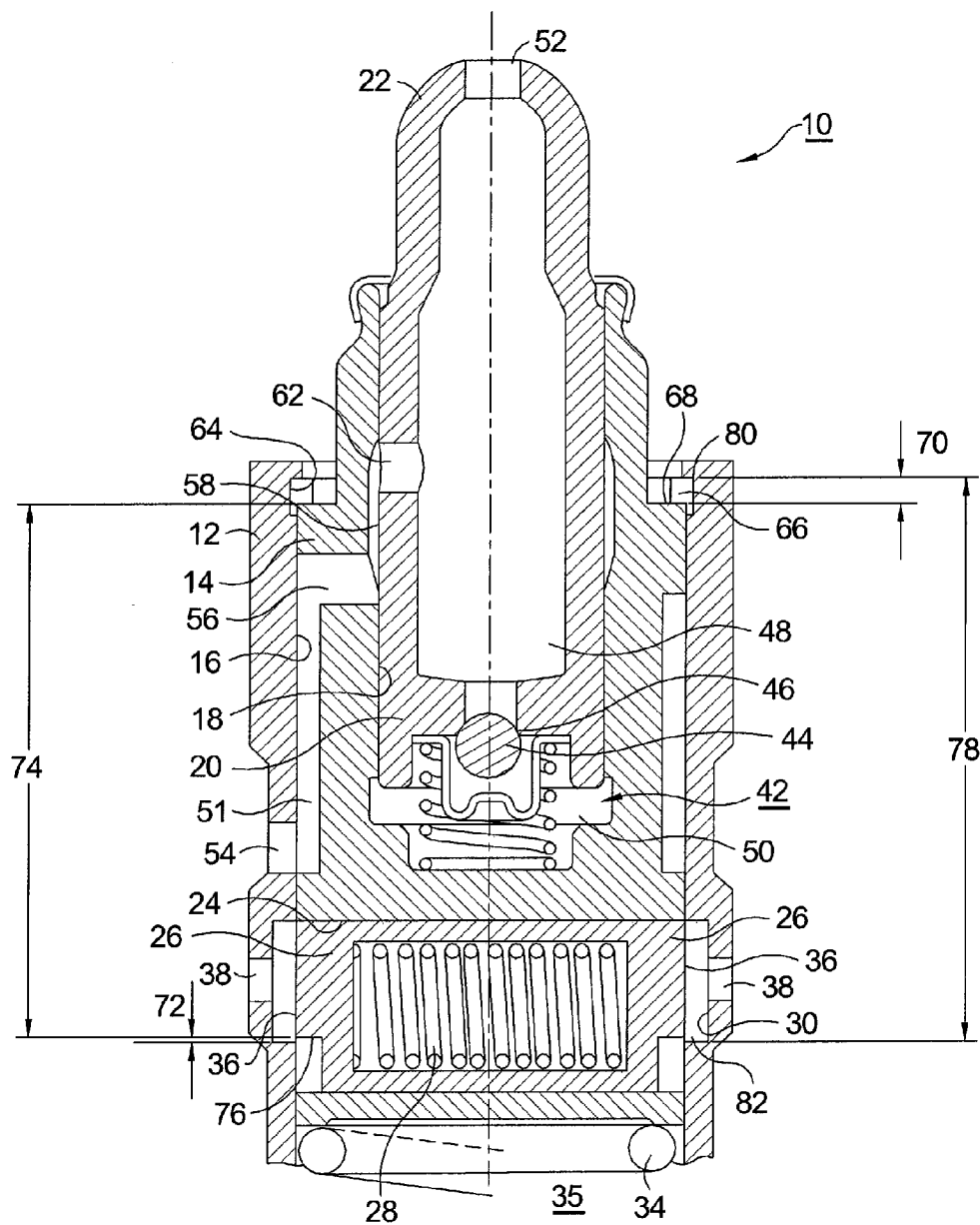
FIG. 1. (PRIOR ART)
