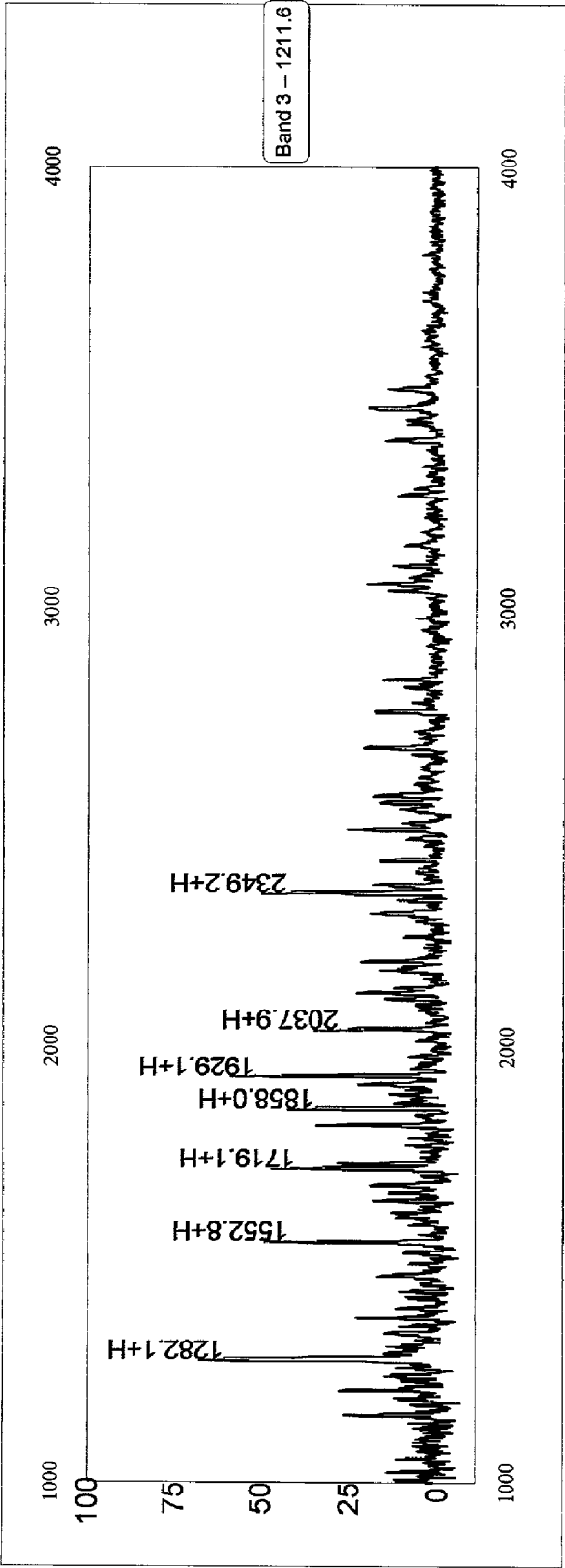
Trypsin Digested Seldi-TOF Spectra FIGURE 2
