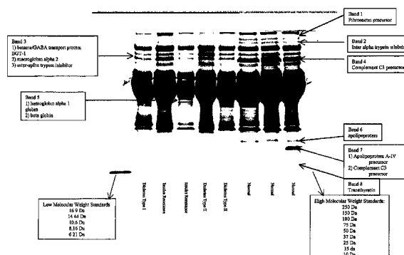
HiQ 1-(Elution) Insulin Resistance vs. Normal
