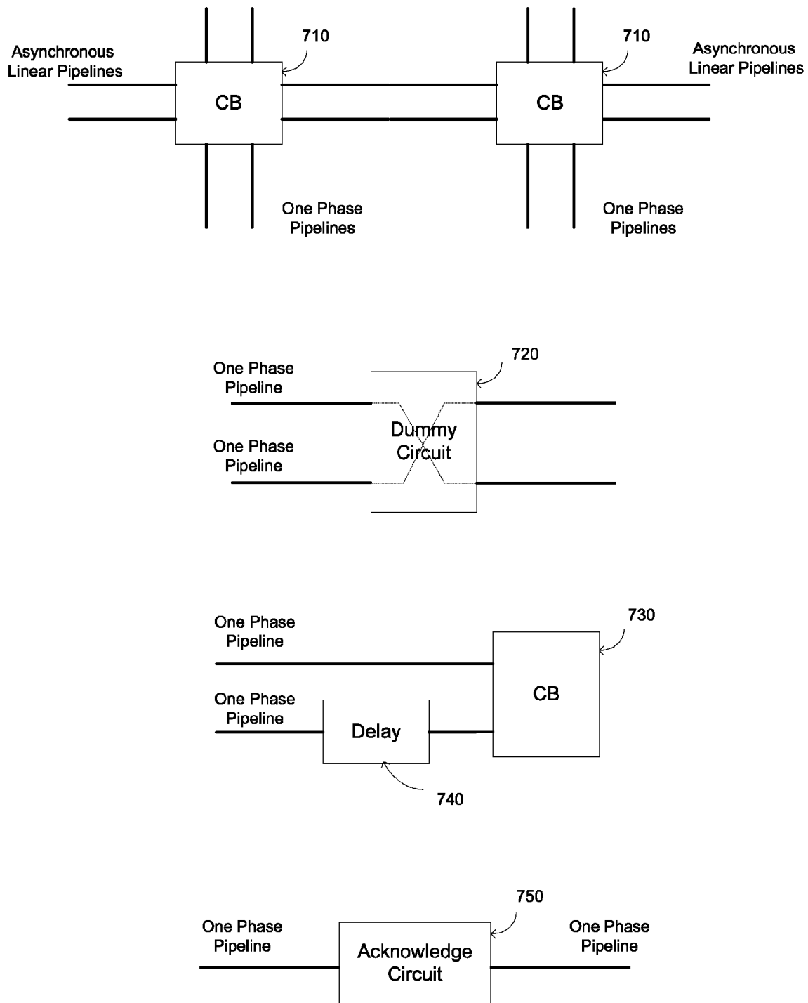
FIG. 7 – Circuit Diagrams
