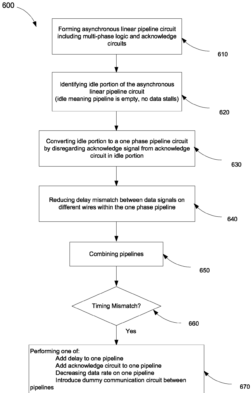
FIG. 6 – Flow Diagram
