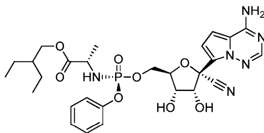
(Compound 1)
