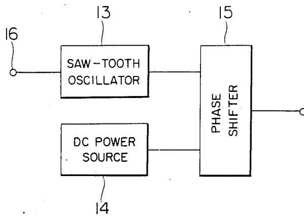
FIG. 2 PRIOR ART
