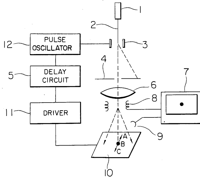
FIG. 2 PRIOR ART
