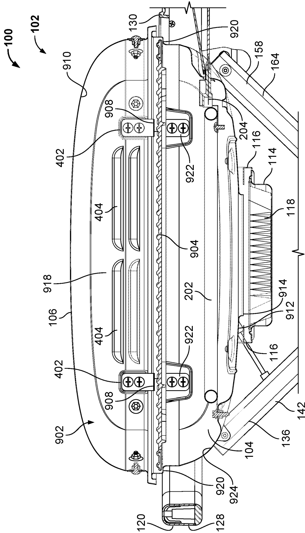
SECTION B-B
