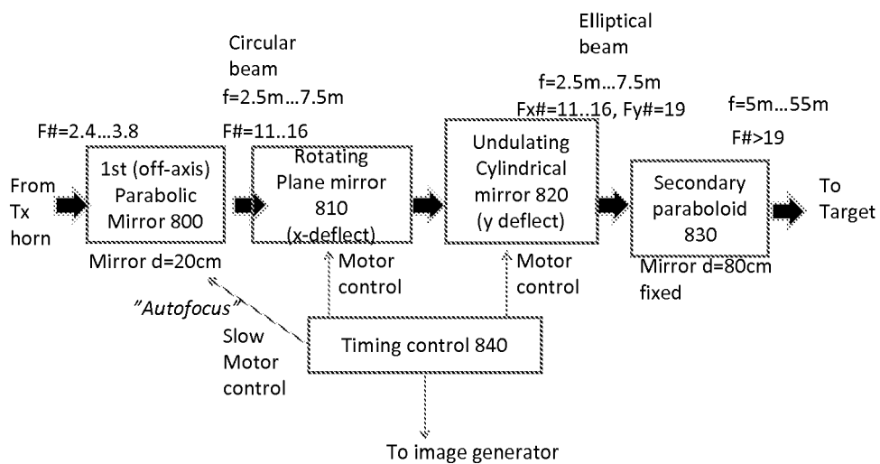
FIG 15 Transmit Beam Scanner
