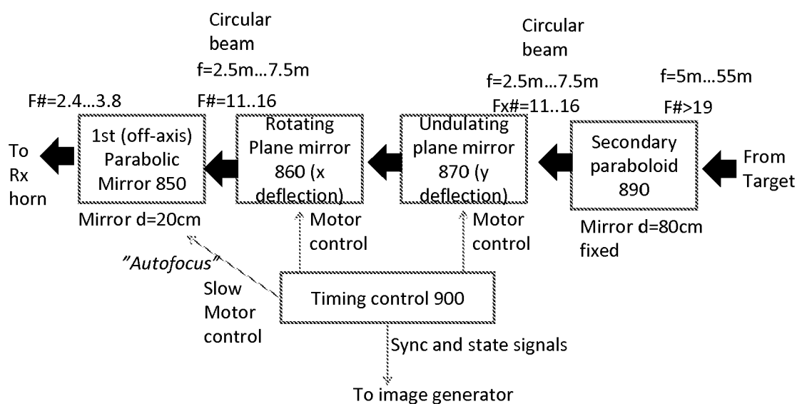
FIG 16 Receive Beam Scanner
