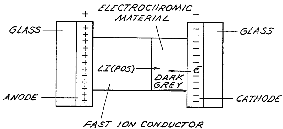
FIG. 3 CATHODIC -5 VOLTS
