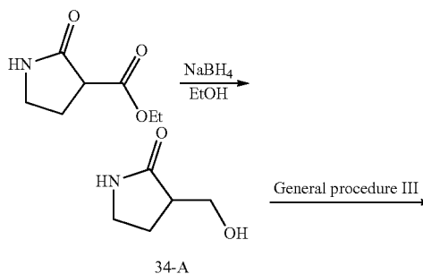
Scheme 19
