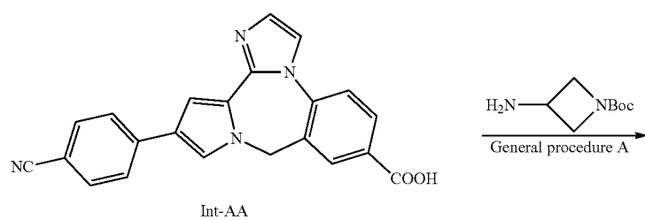
Scheme 60
