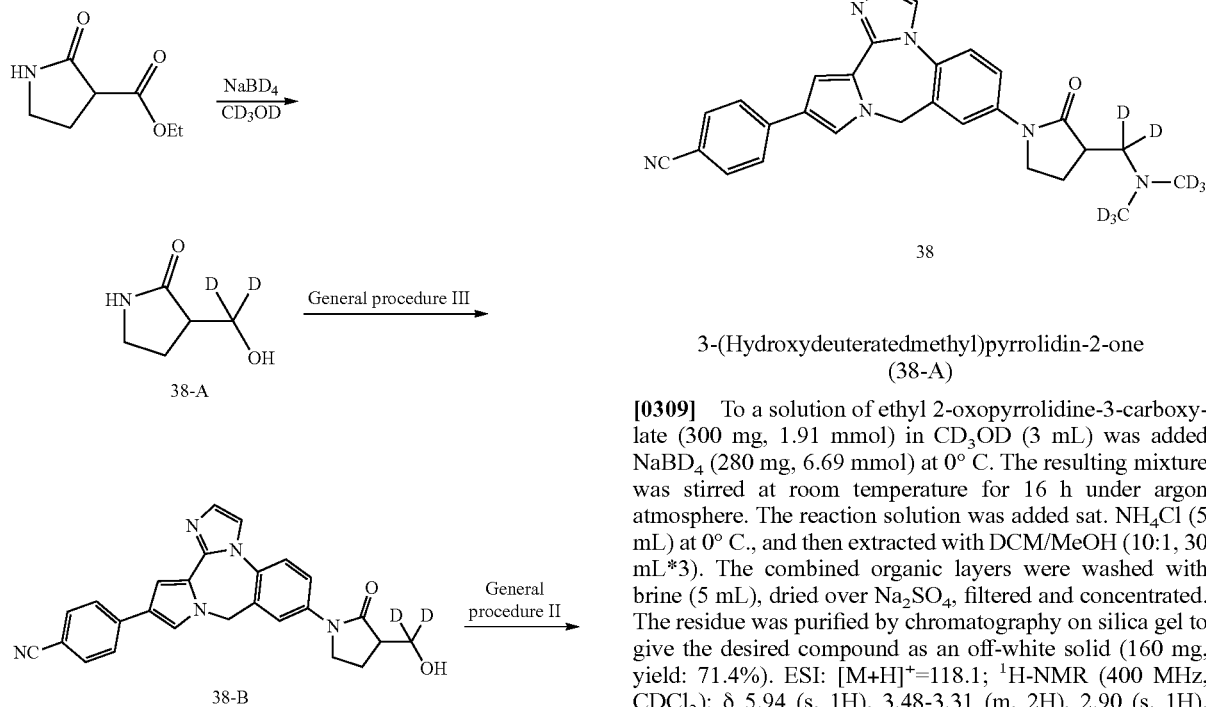
Scheme 21
