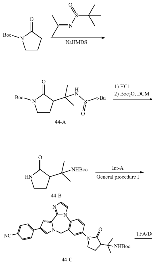
Scheme 25
