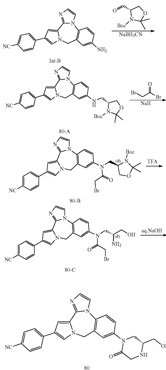
Scheme 47
