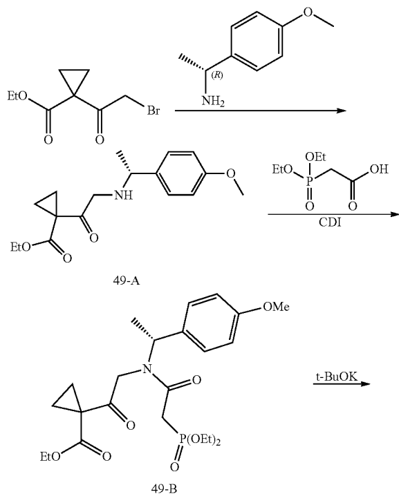
Scheme 29
