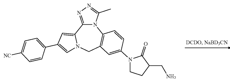
Scheme 50
