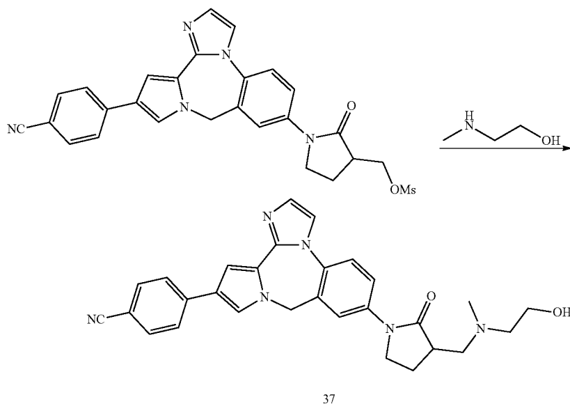
Scheme 20
