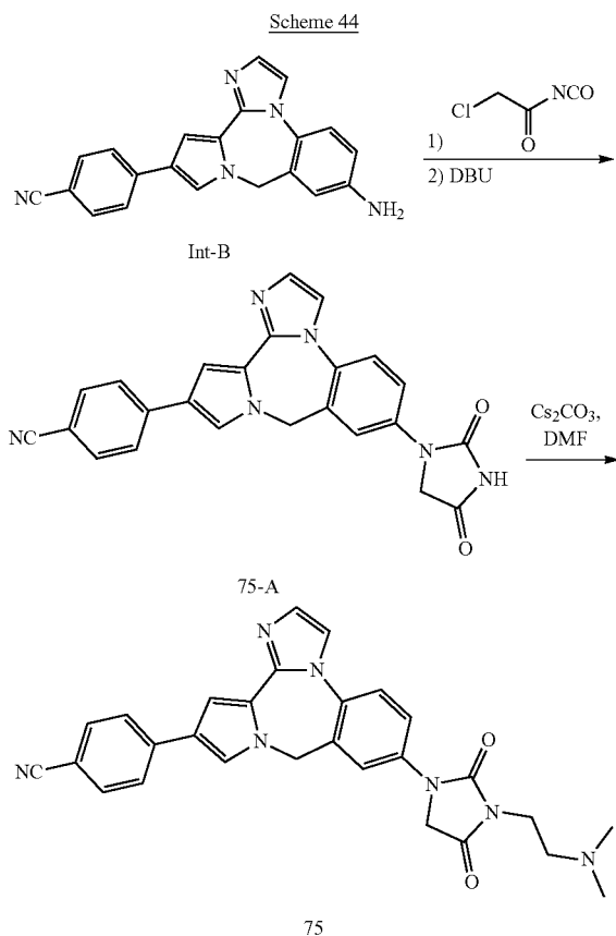
4-(7-(2,4-Dioxoimidazolidin-1-yl)-9H-benzo[e]imidazo[2,1-c]pyrrolo[1,2-a][1,4]diazepin-12-yl)benzonitrile (75-A)
