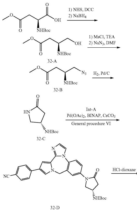
Scheme 17
