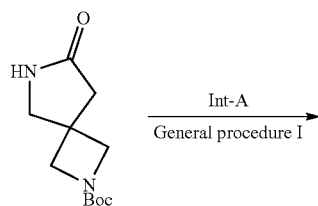
Scheme 10
