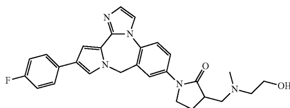
Scheme 54
