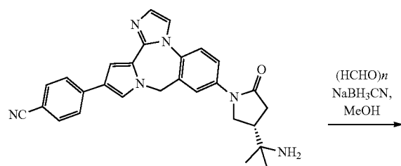
Scheme 30
