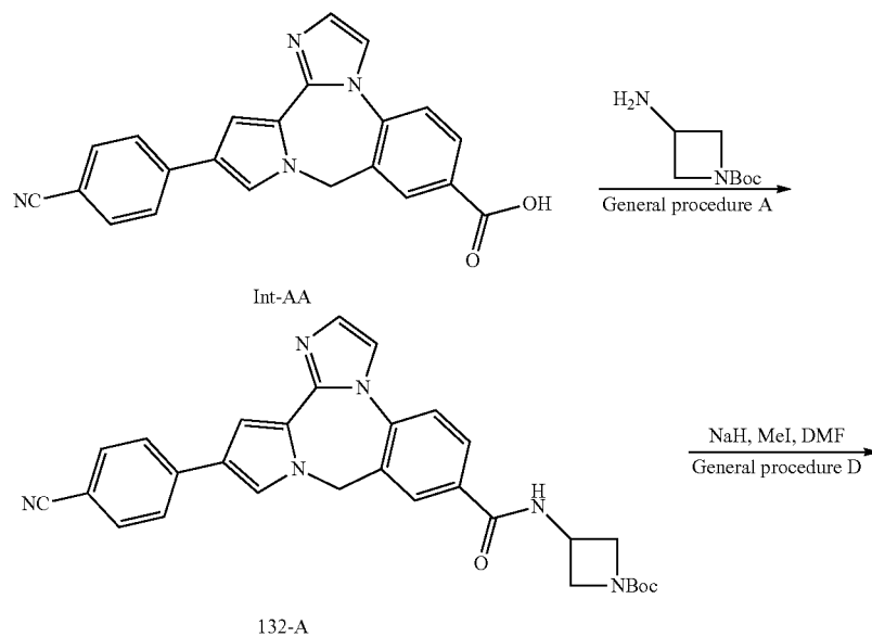
Scheme 62
