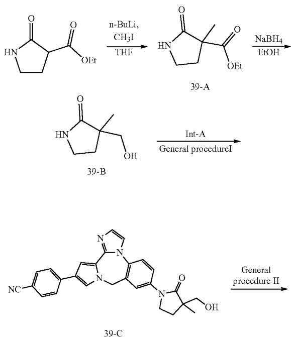
Scheme 22
