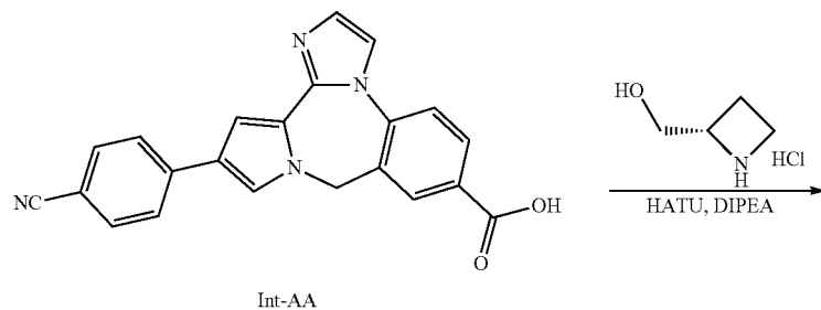
Scheme 64
