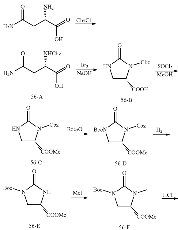
Scheme 32
