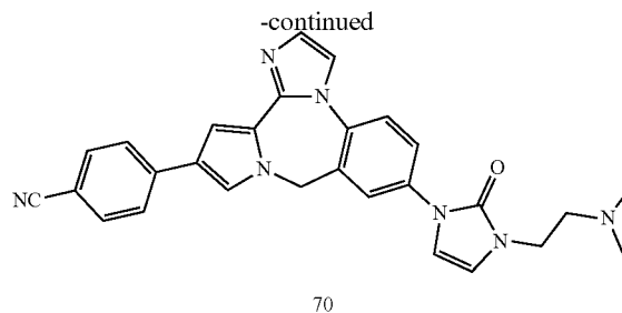
4-(7-((Diphenylmethylene)amino)-9H-benzo[e]imidazo[2,1-c]pyrrolo[1,2-a][1,4]diazepin-12-yl)benzonitrile (Int-B-1)
