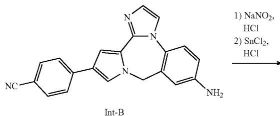
Scheme 46
