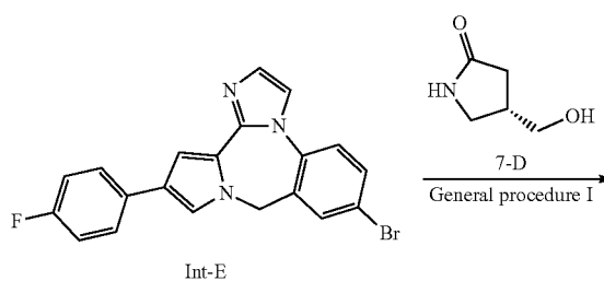
Scheme 53
