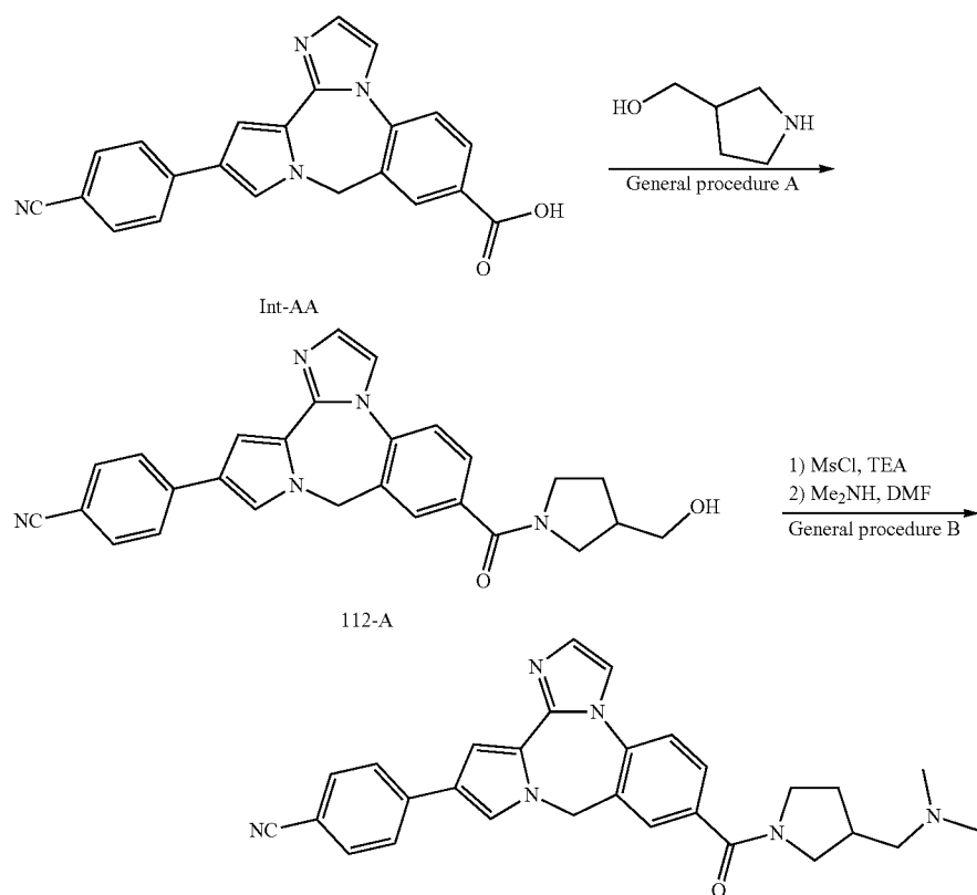
Scheme 59
