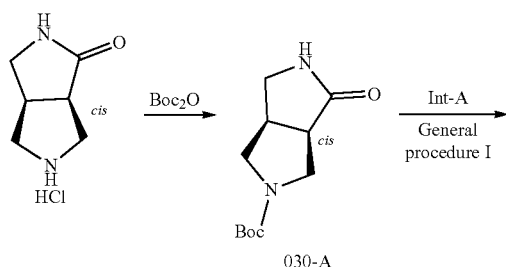
Scheme 15
