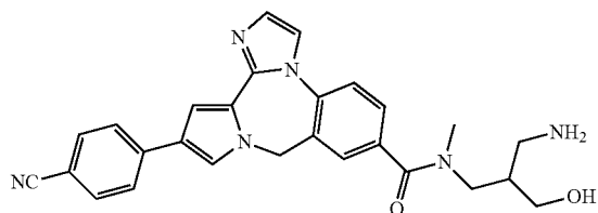
Scheme 63
