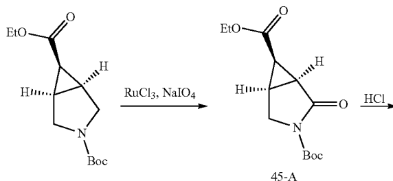
Scheme 26
