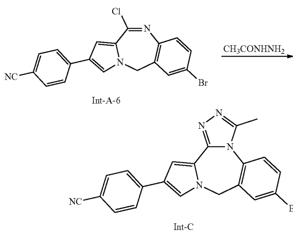
Scheme 48
