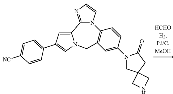
Scheme 11
