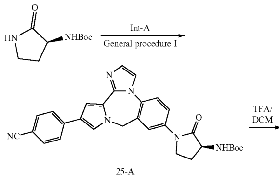
Scheme 13
