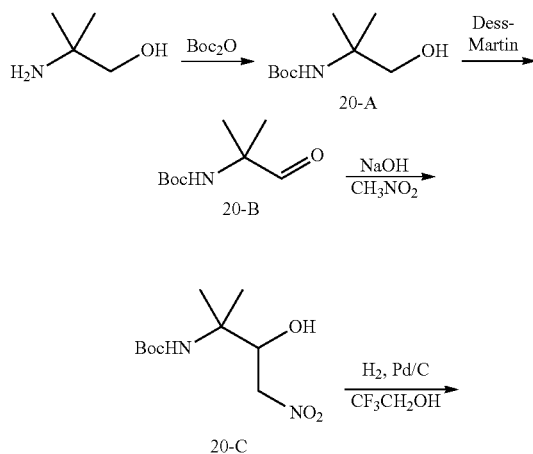
Scheme 8
