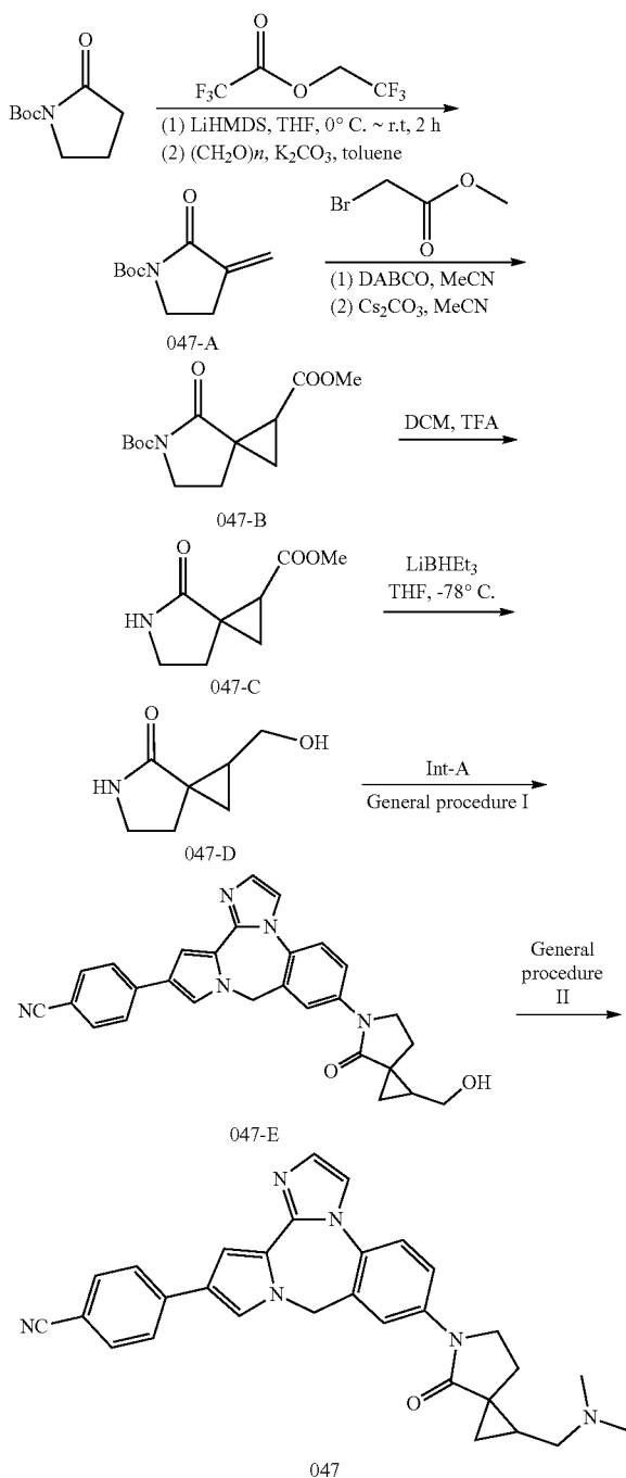
Scheme 27
