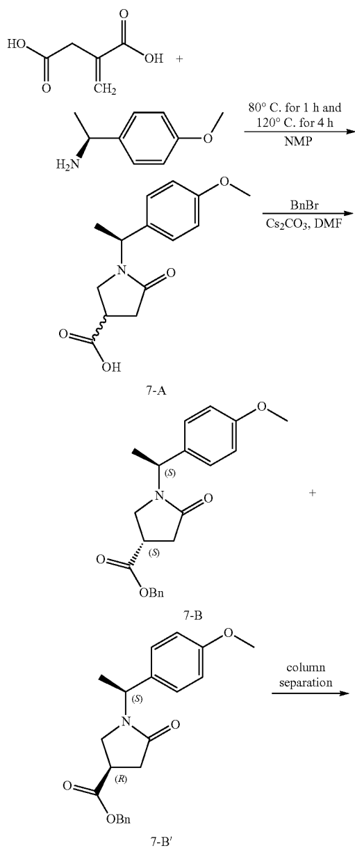
Scheme 4
