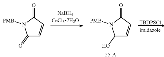
Scheme 31
