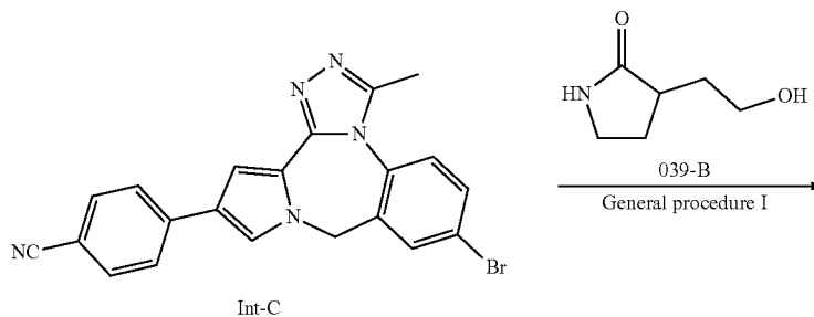
Scheme 49
