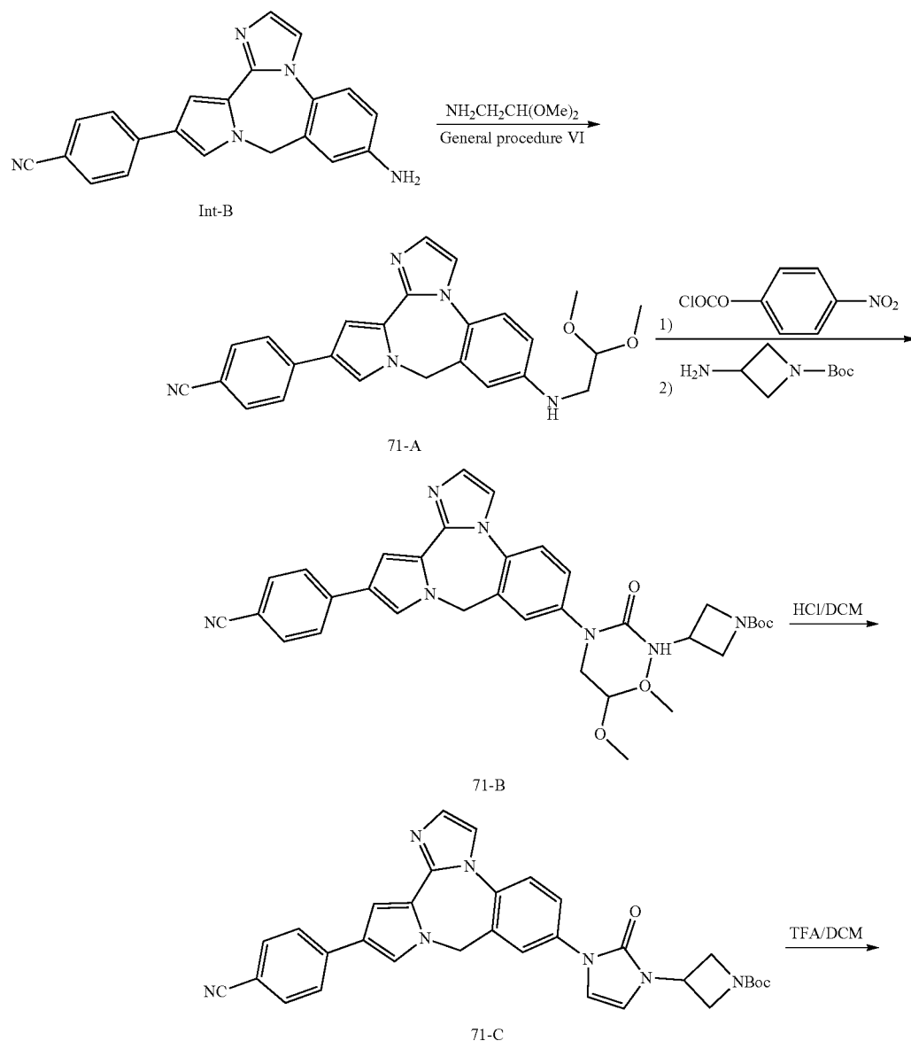
Scheme 42
