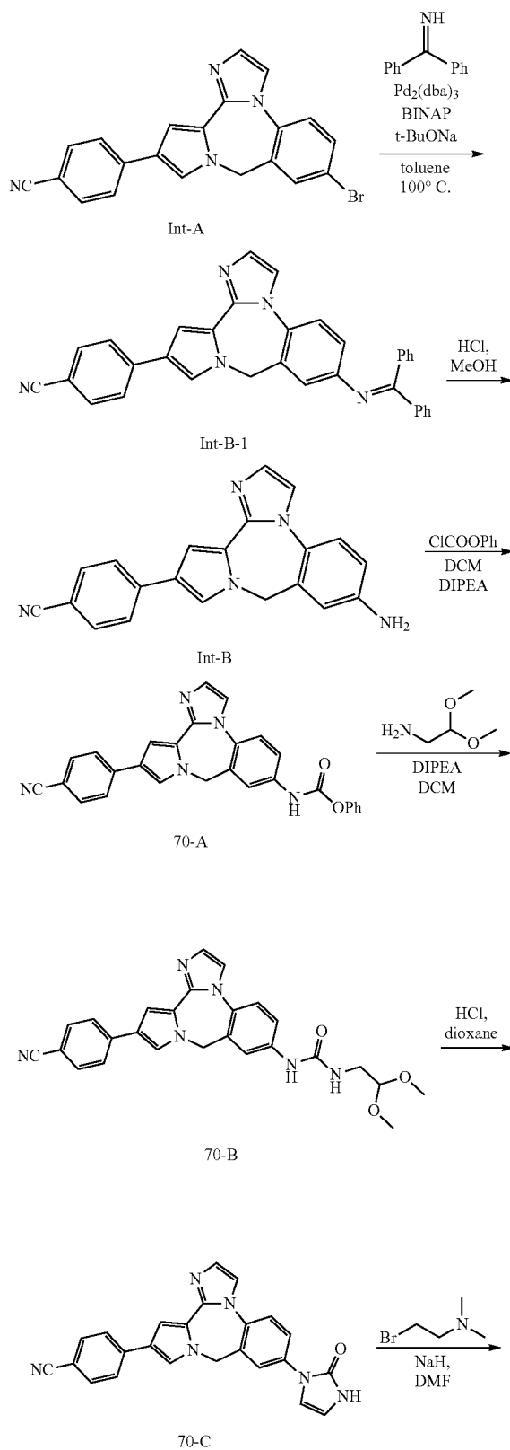
Scheme 41
