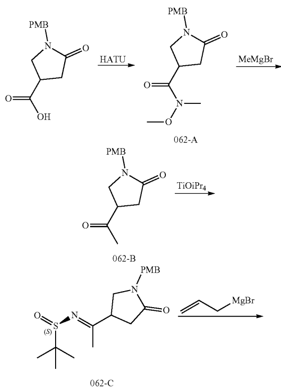
Scheme 38
