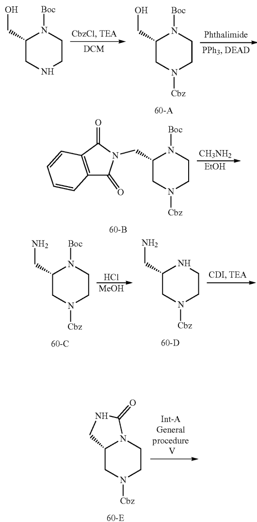
Scheme 36
