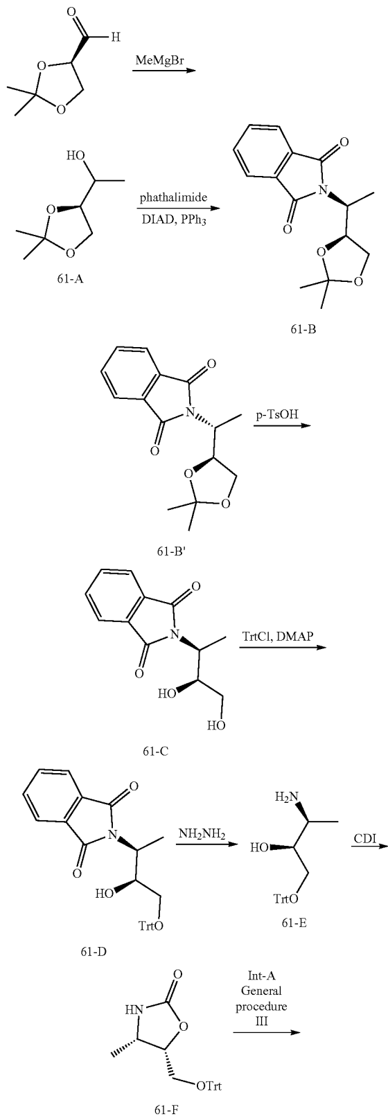
Scheme 37
