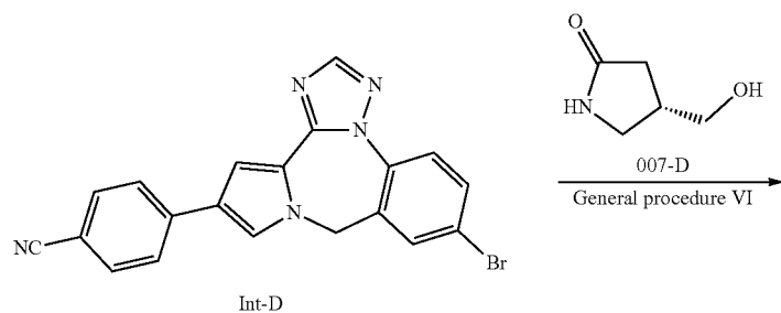
Scheme 52
