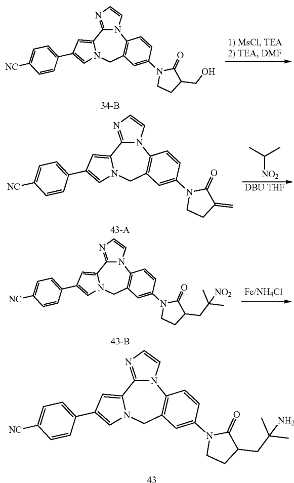
Scheme 24
