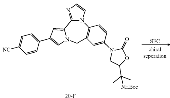
Scheme 9
