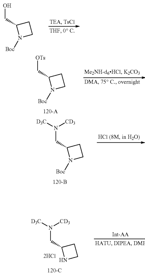
Scheme 61
