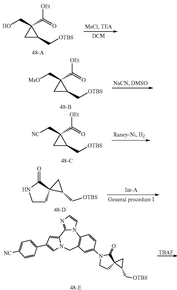
Scheme 28
