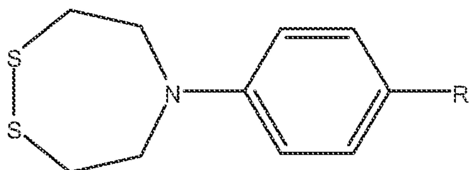
Structure 6
