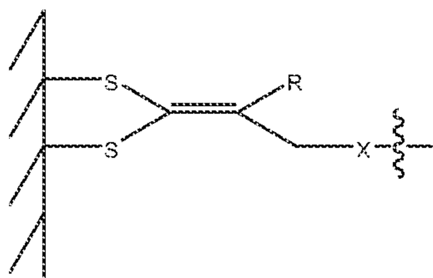
Structure 4
