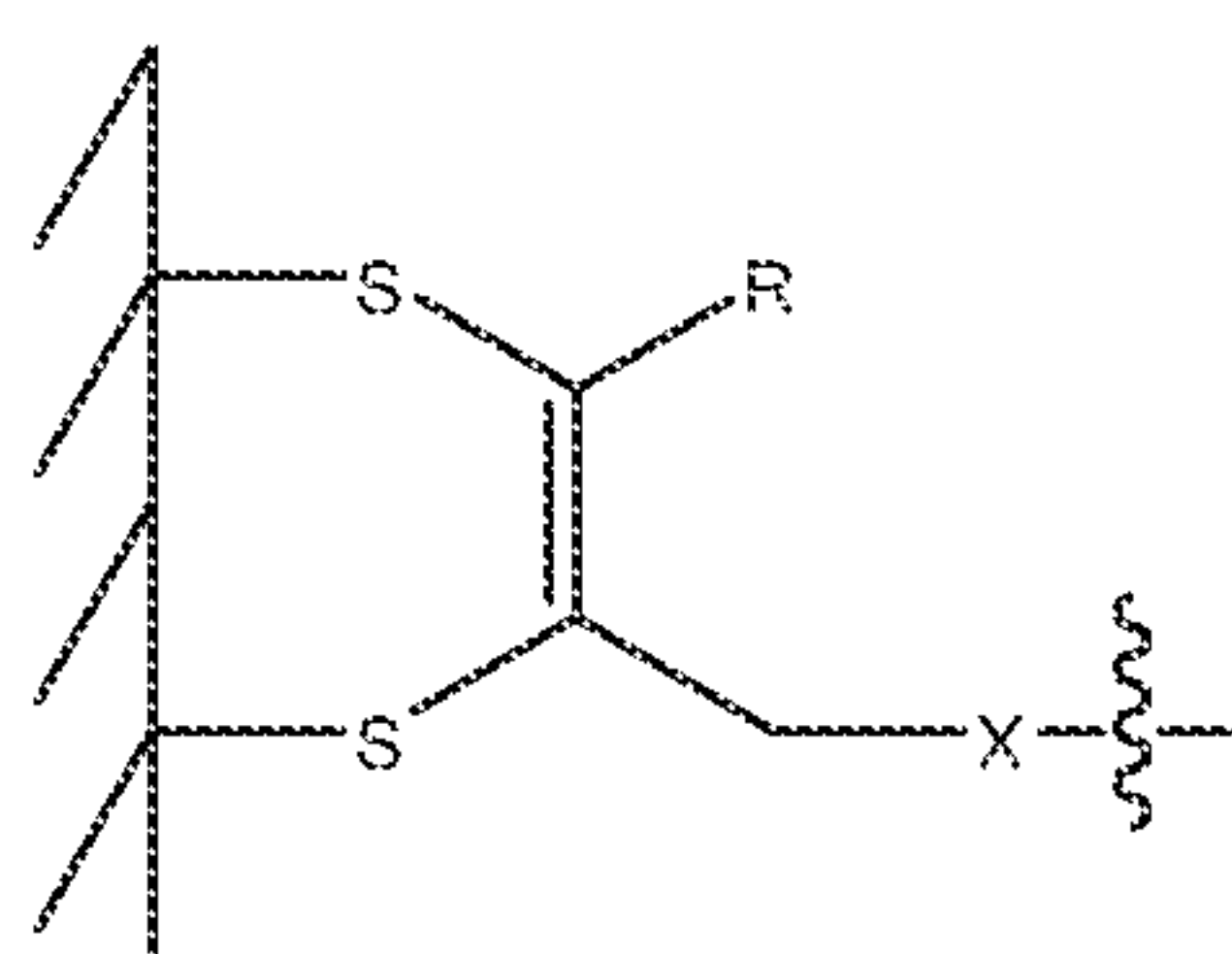
Structure 3
