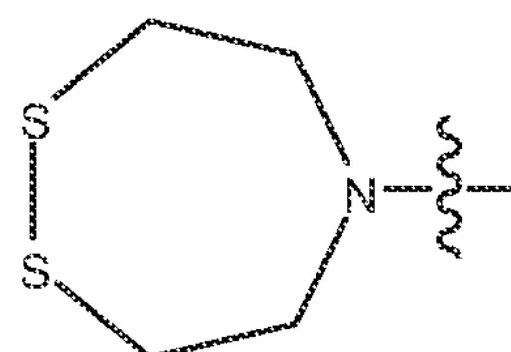
Structure 5
