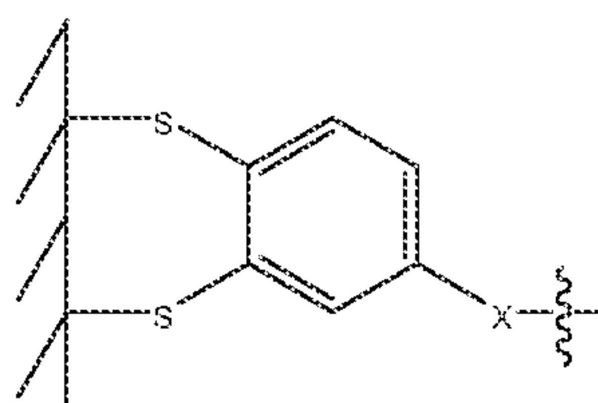
Structure 3
