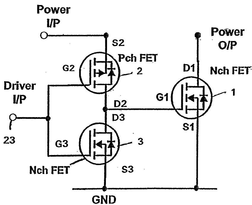
FIGURE 7 (INVERTING DRIVE)
