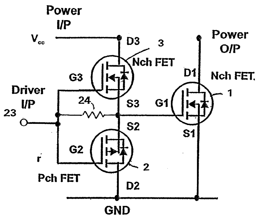
FIGURE 1 (NON INVERTING DRIVE)
