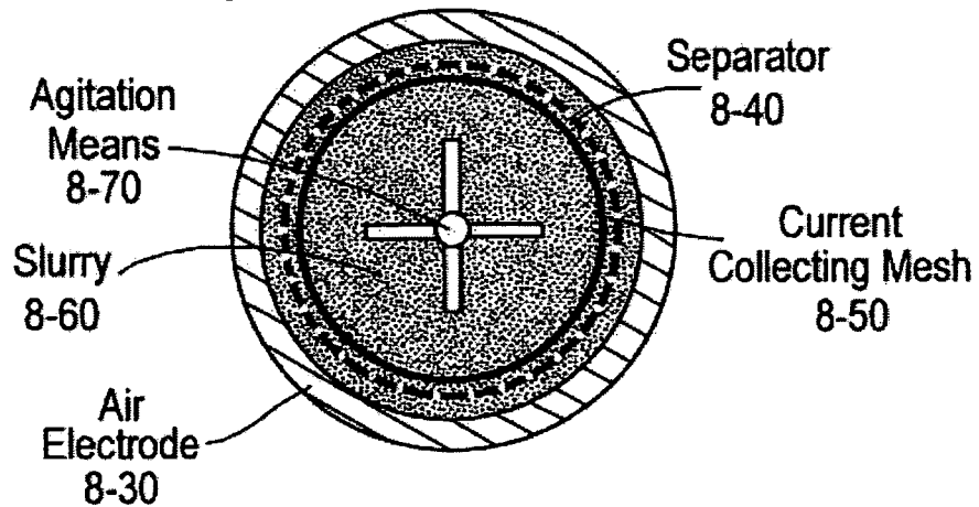
Top View Schematic
