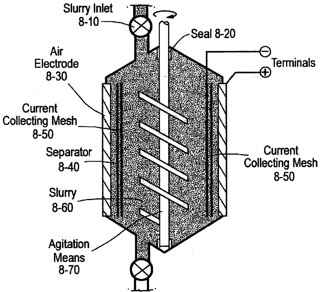
Side View Schematic
